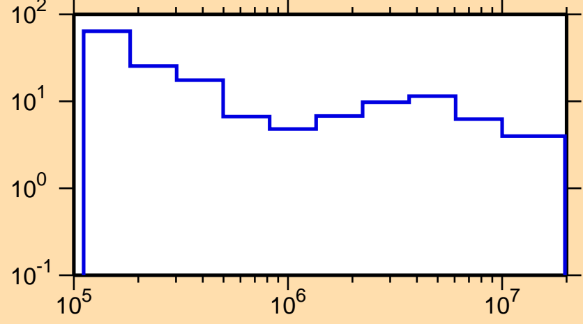
\Delta\sigma/\sigma vs. E for ^{145}\text{Ba}(n,\text{tot.})
