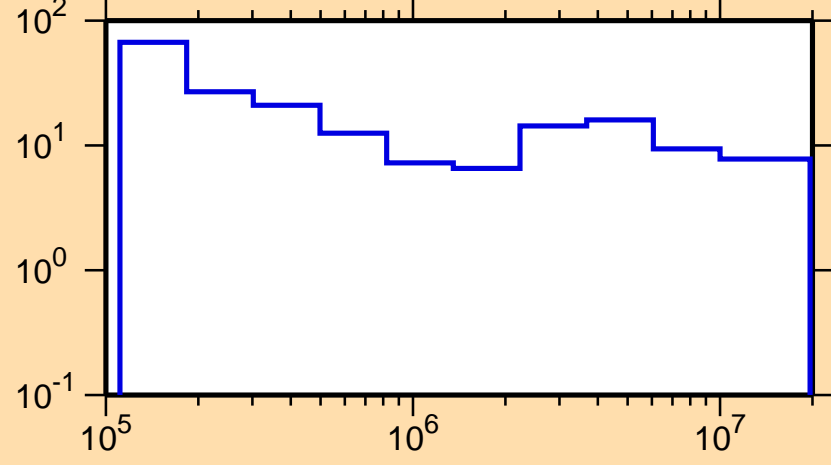
\Delta\sigma/\sigma vs. E for ^{145}\text{Ba}(n,\text{el.})
