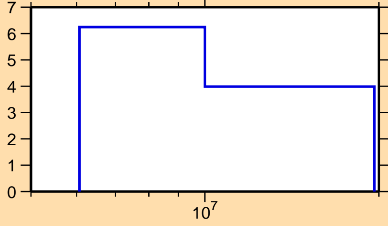
\Delta\sigma/\sigma vs. E for ^{145}\text{Ba}(n,\text{tot.})
