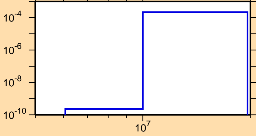
\sigma vs. E for ^{145}\text{Ba}(n,p)
