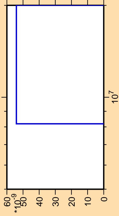
\Delta\sigma/\sigma vs. E for ^{145}\text{Ba} (mt 11)
