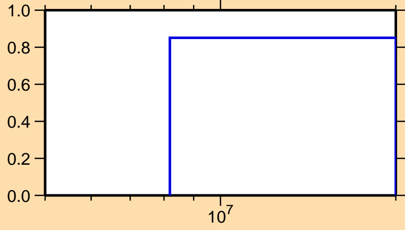
\sigma vs. E for ^{145}\text{Ba}(n,3n)
