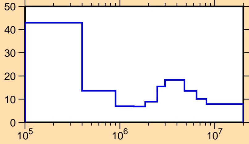
\Delta\sigma/\sigma vs. E for ^{145}\text{Ba}(n,\text{el.})
