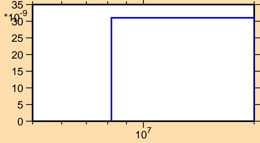
\sigma vs. E for ^{145}\text{Ba}(n,2n\alpha)
