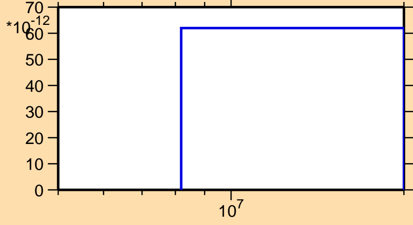
\sigma vs. E for ^{145}\text{Ba}(n,2np)
