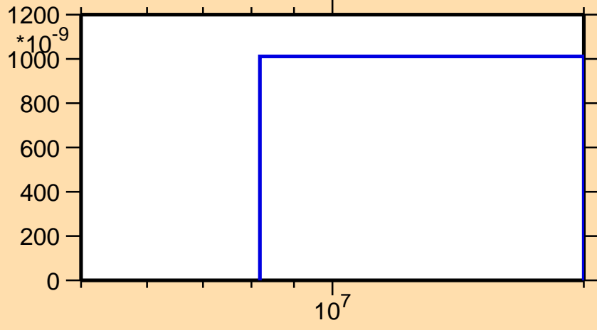
\sigma vs. E for ^{145}\text{Ba}(n,np)
