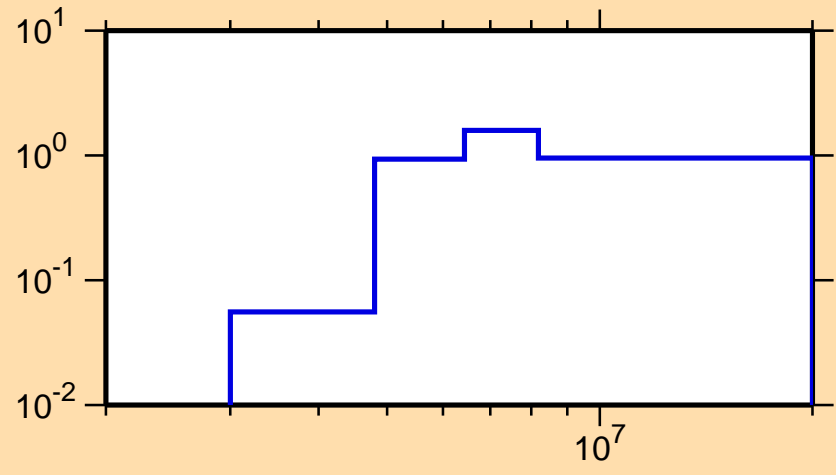
\sigma vs. E for ^{145}\text{Ba}(n,2n)
