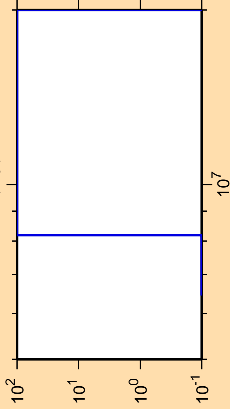
\Delta\sigma/\sigma vs. E for ^{145}\text{Ba}(n,p)
