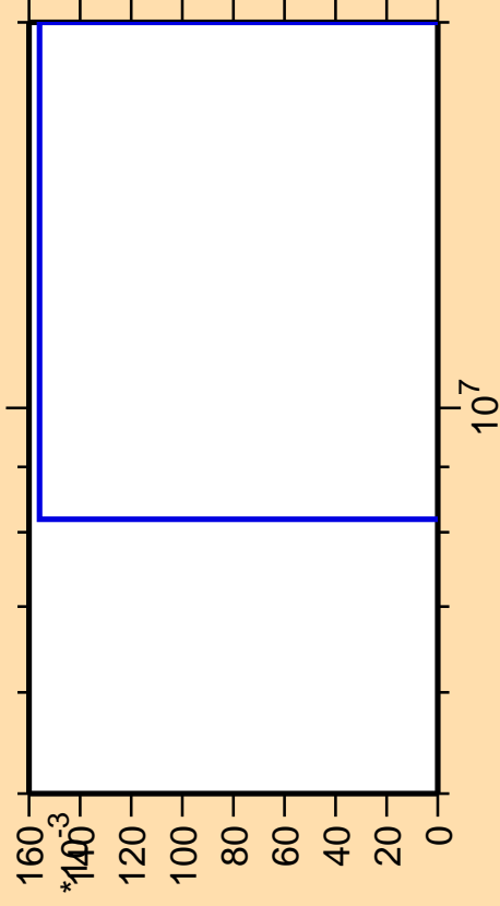
\Delta\sigma/\sigma vs. E for ^{145}\text{Ba}(n,3n\alpha)
