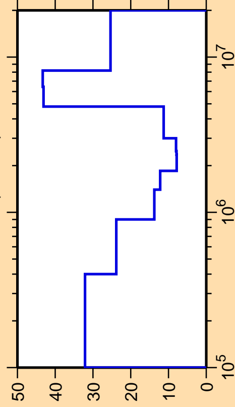
\Delta\sigma/\sigma vs. E for ^{145}\text{Ba}(n,\text{inel.})
