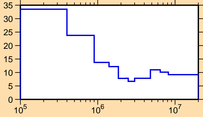
\Delta\sigma/\sigma vs. E for ^{145}\text{Ba}(n,\text{nonel.})
