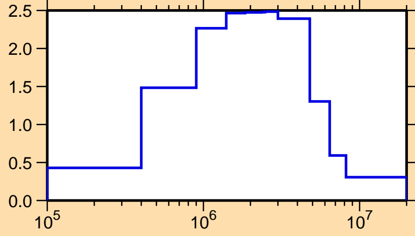
\sigma vs. E for ^{145}\text{Ba}(n,\text{inel.})
