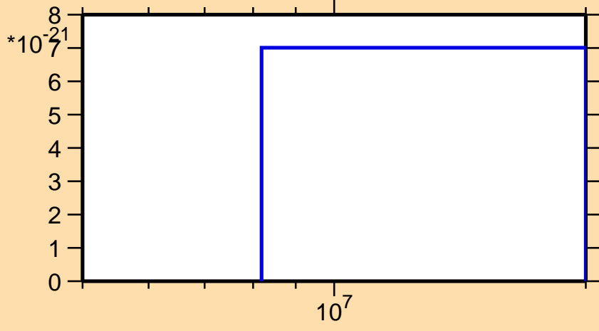
\sigma vs. E for ^{145}\text{Ba} (mt 11)
