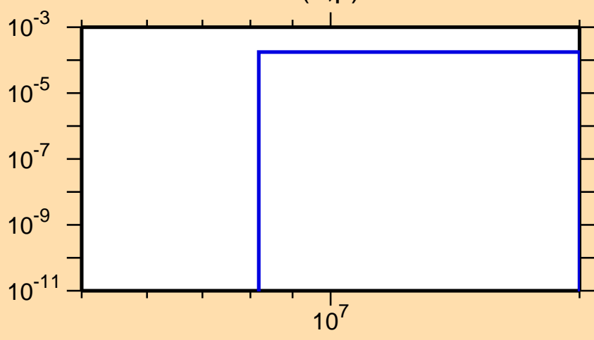
\sigma vs. E for ^{145}\text{Ba}(n,p)
