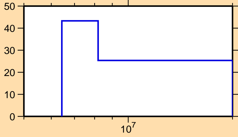
\Delta\sigma/\sigma vs. E for ^{145}\text{Ba}(n,\text{inel.})
