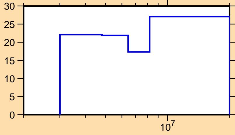
\Delta\sigma/\sigma vs. E for ^{145}\text{Ba}(n,2n)
