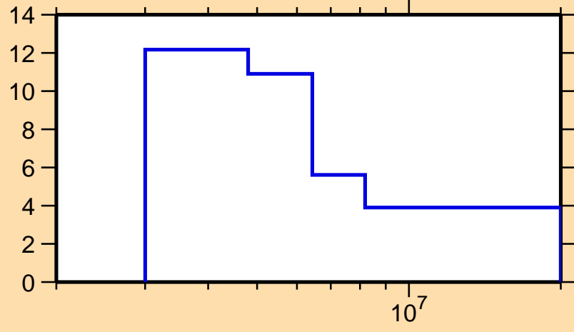
\Delta\sigma/\sigma vs. E for ^{145}\text{Ba}(n,\text{tot.})
