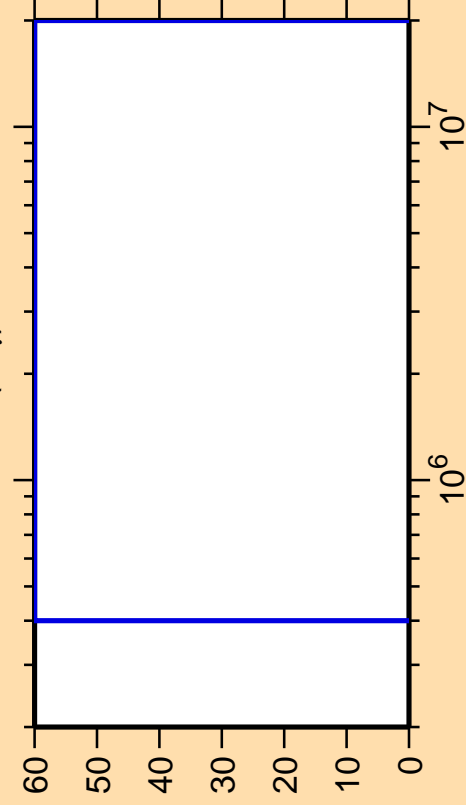
\Delta\sigma/\sigma vs. E for ^{145}\text{Ba}(n,\gamma)
