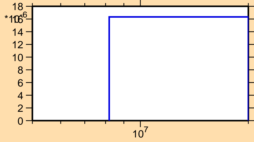
\sigma vs. E for ^{145}\text{Ba}(n,n\alpha)
