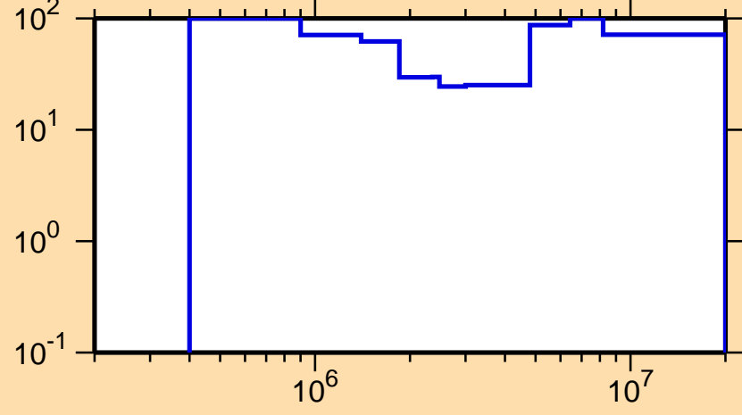
\Delta\sigma/\sigma vs. E for ^{145}\text{Ba}(n,n\text{cont.})
