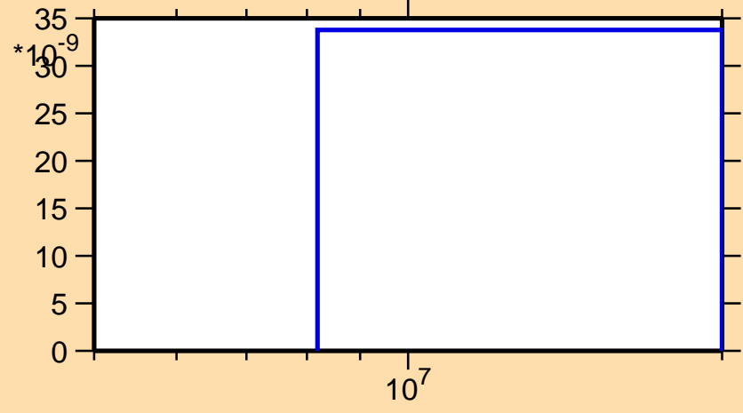
\sigma vs. E for ^{145}\text{Ba}(n,\text{nt})
