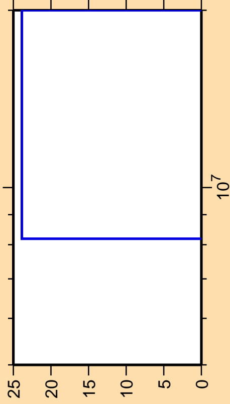
\Delta\sigma/\sigma vs. E for ^{145}\text{Ba}(n,3n)
