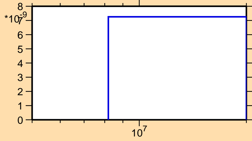
\sigma vs. E for ^{145}\text{Ba}(n,\text{nd})
