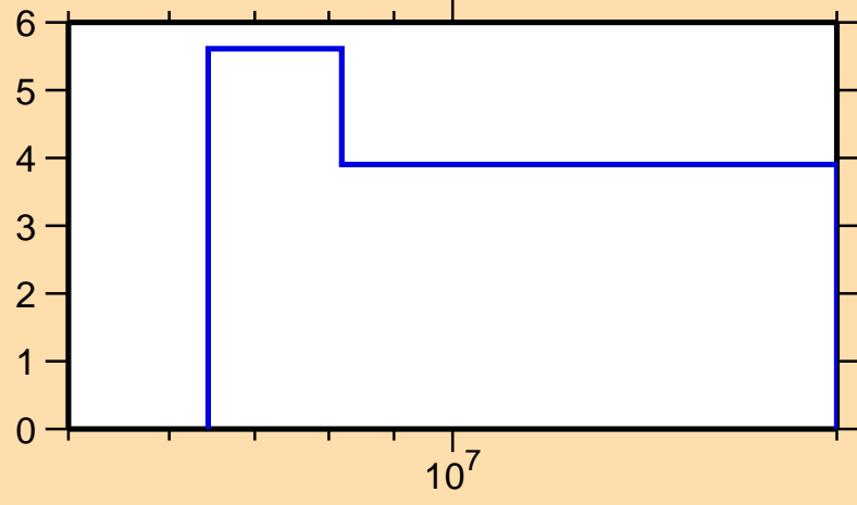
\Delta\sigma/\sigma vs. E for ^{145}\text{Ba}(n,\text{tot.})
