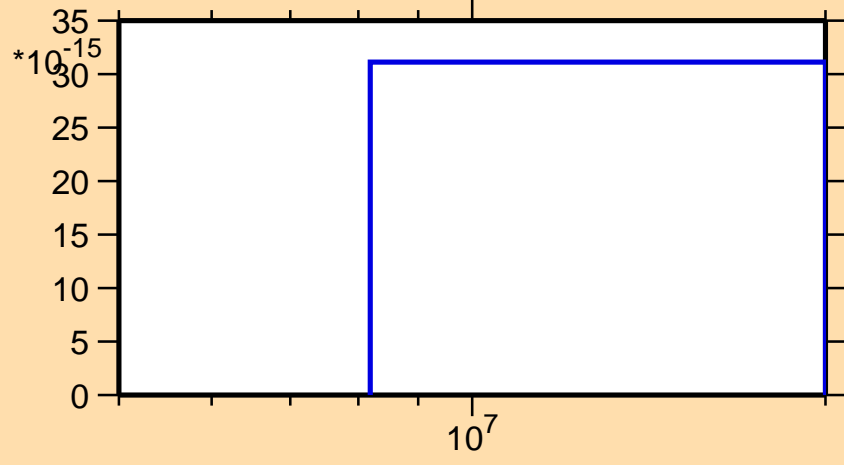
\sigma vs. E for ^{145}\text{Ba}(n,3n\alpha)
