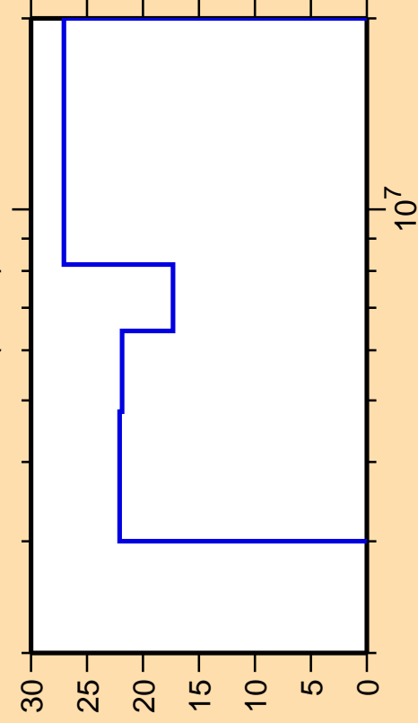
\Delta\sigma/\sigma vs. E for ^{145}\text{Ba}(n,2n)
