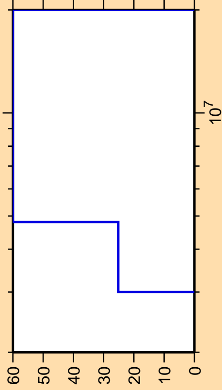
\Delta\sigma/\sigma vs. E for ^{145}\text{Ba}(n,n\text{cont.})
