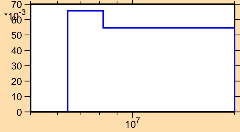
\sigma vs. E for ^{10}\text{Be}(n,n_3)
