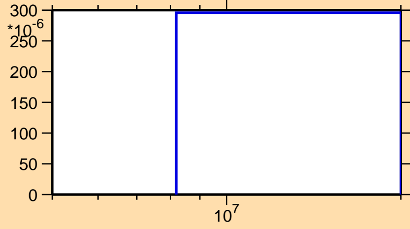
\sigma vs. E for ^{10}\text{Be}(n,n\text{cont.})
