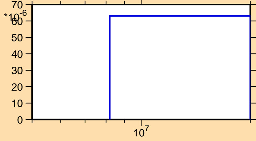
\sigma vs. E for ^{10}\text{Be}(n,t)
