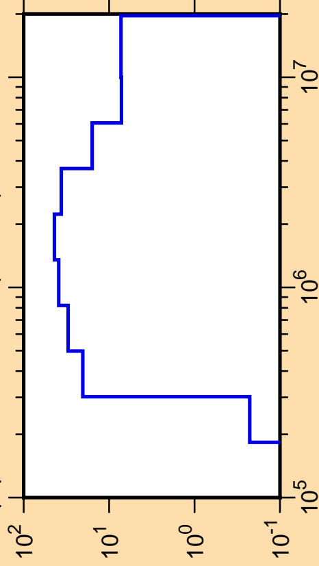
\Delta\mu/\mu vs. E for ^{11}\text{Be}(\text{mt251})
