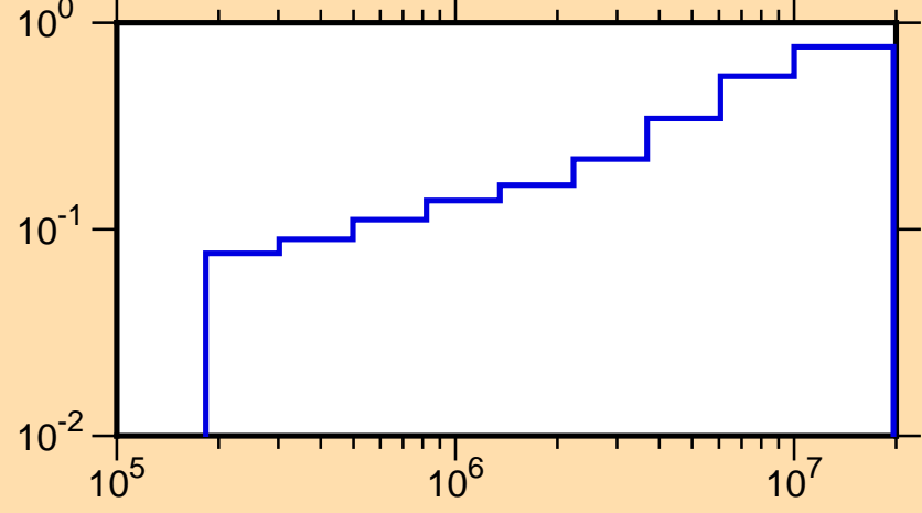
\mu vs. E for ^{11}\text{Be}(\text{mt251})
