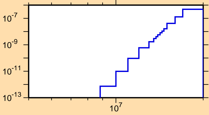
\sigma vs. E for ^{264}\text{He3}
