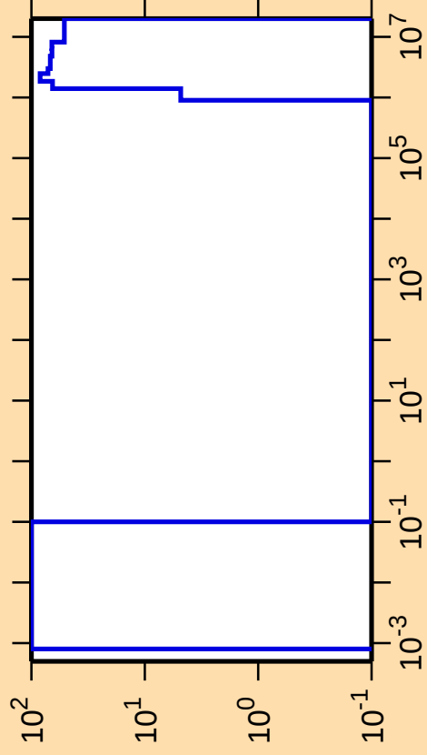
\Delta\sigma/\sigma vs. E for ^{272}\text{Zr}
