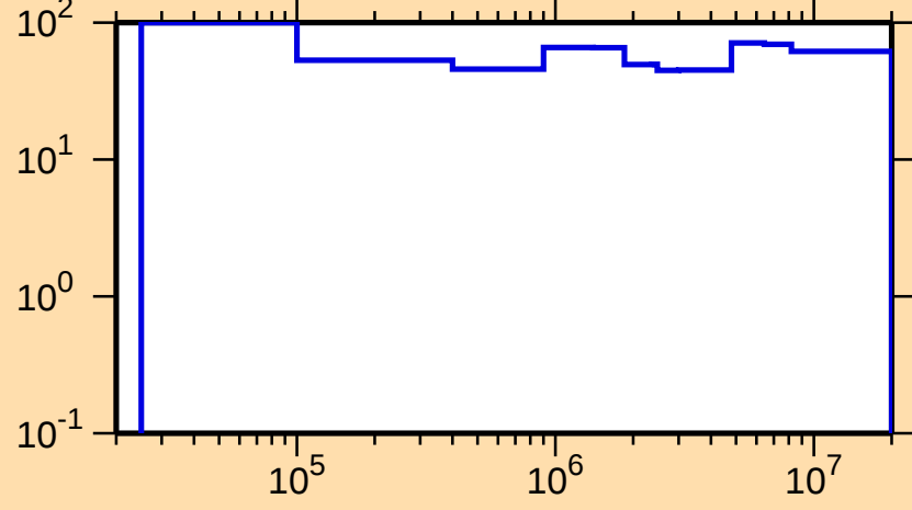
\Delta\sigma/\sigma vs. E for ^{272}_1 )
