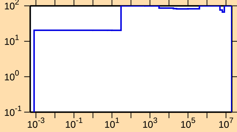
\Delta\sigma/\sigma vs. E for ^{272}\text{Zr}
