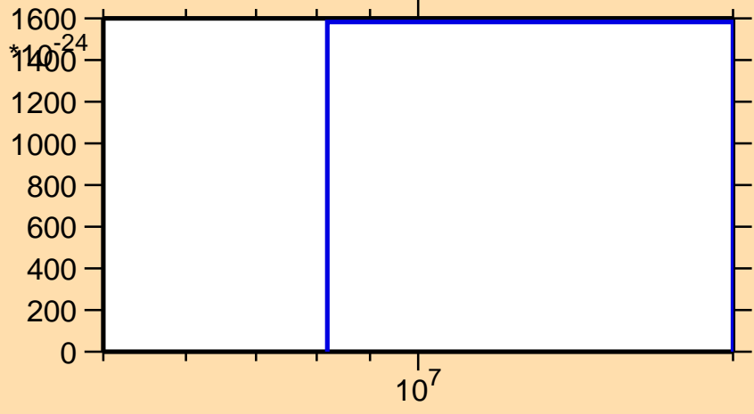
\sigma vs. E for ^{190}\text{Bi}(\text{mt } 42)
