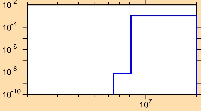
\sigma vs. E for ^{190}\text{Bi}(n,t)
