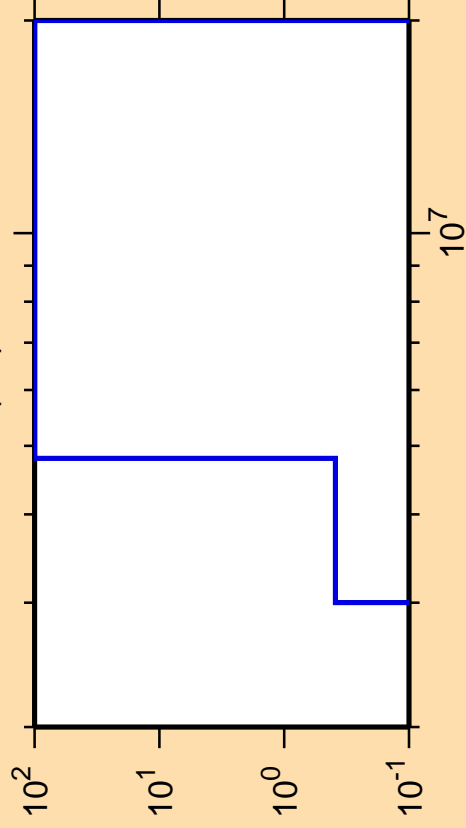
\Delta\sigma/\sigma vs. E for ^{190}\text{Bi}(n,t)
