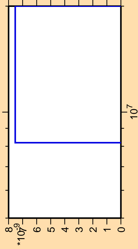
\Delta\sigma/\sigma vs. E for ^{190}\text{Bi}(\text{mt } 42)
