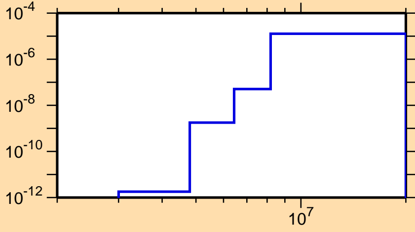
\sigma vs. E for ^{191}\text{Bi} (mt 45)
