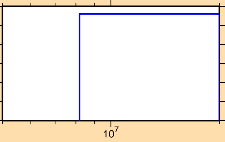
\sigma vs. E for ^{191}\text{Bi}(n,\text{nd})
