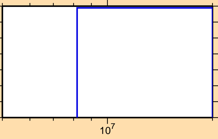
\sigma vs. E for ^{191}\text{Bi}(n,\text{pd})
