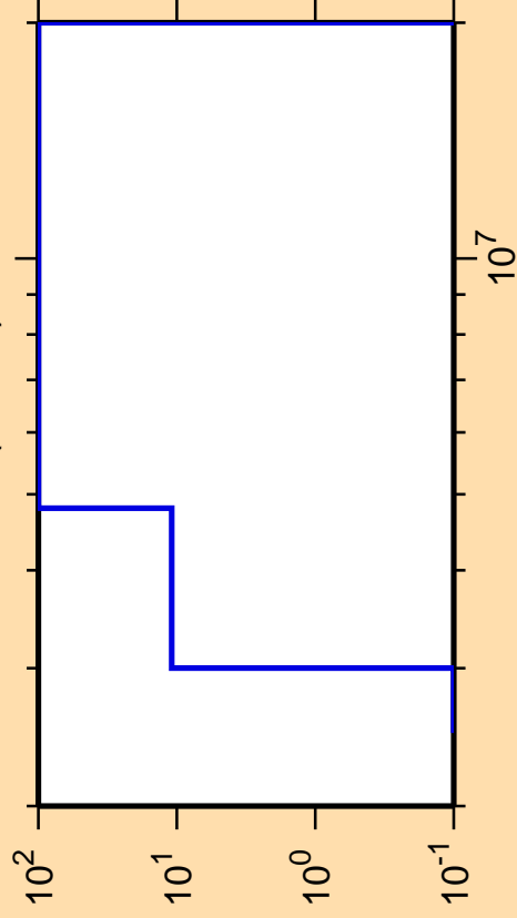
\Delta\sigma/\sigma vs. E for ^{191}\text{Bi} (mt 45)
