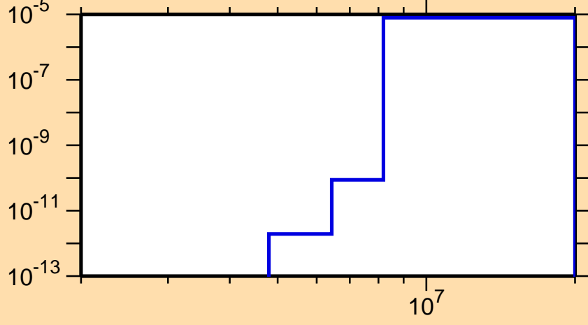
\sigma vs. E for ^{191}\text{Bi}(n,\text{He}3)
