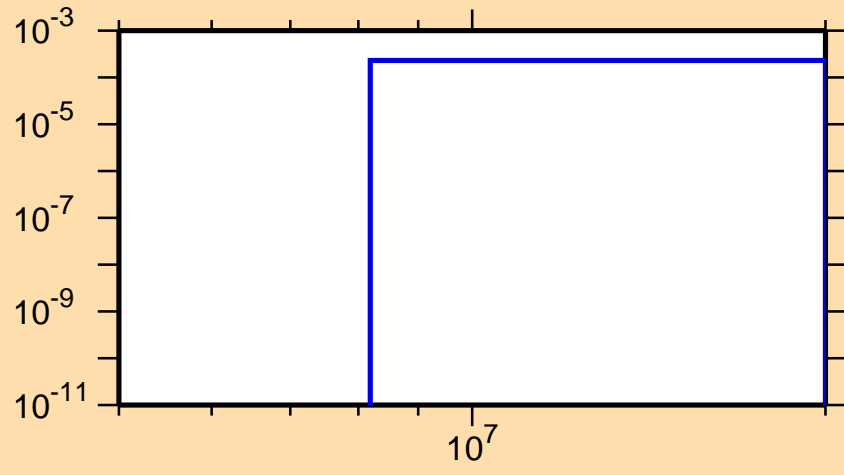
\sigma vs. E for ^{191}\text{Bi}(n,t)
