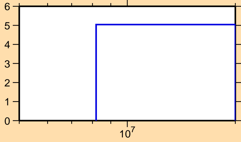
\Delta\sigma/\sigma vs. E for ^{191}\text{Bi}(n,\text{el.})
