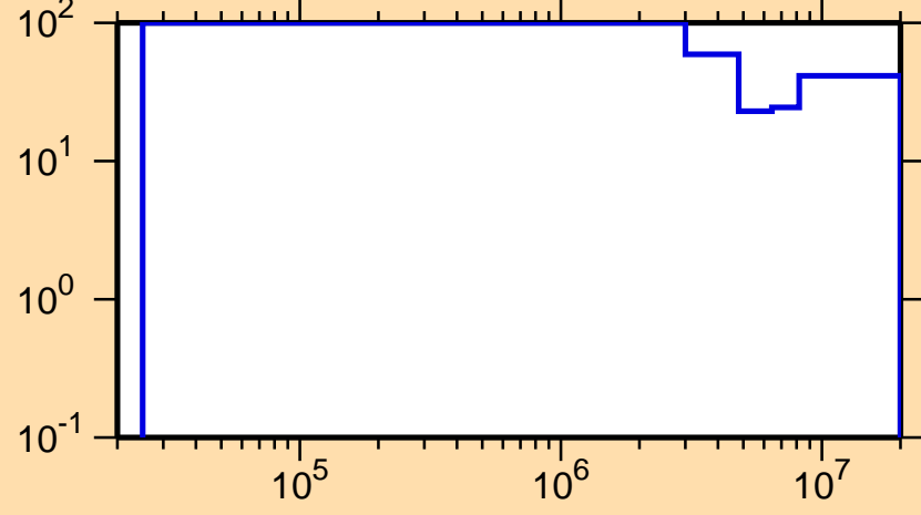
\Delta\sigma/\sigma vs. E for ^{192}\text{Bi}(n,n\text{cont.})
