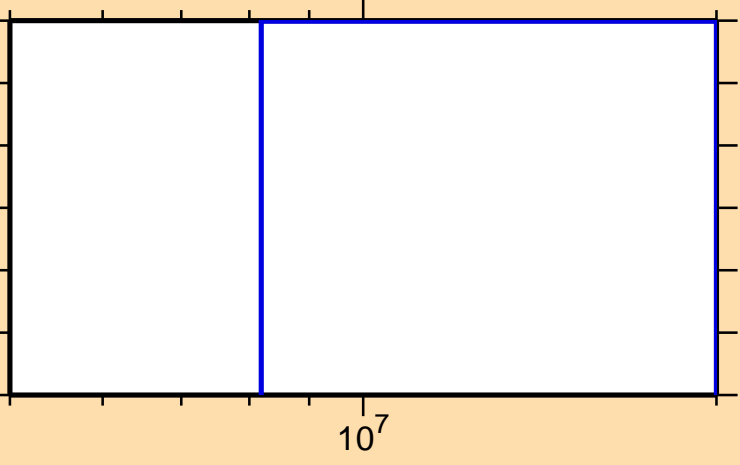
\sigma vs. E for ^{192}\text{Bi}(n,2n\alpha)
