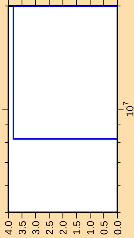
\Delta\sigma/\sigma vs. E for ^{193}\text{Bi}(\text{mt } 34)
