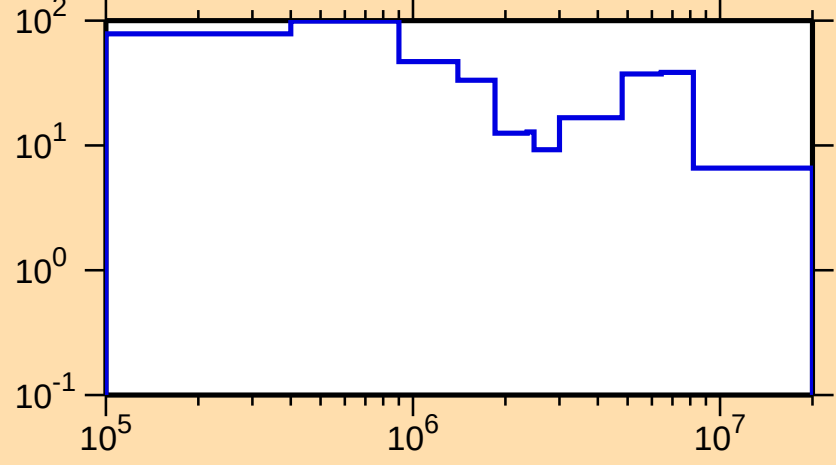
\Delta\sigma/\sigma vs. E for ^{193}\text{Bi}(n,\text{el.})
