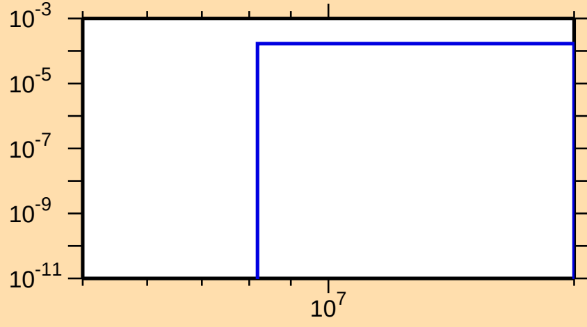
\sigma vs. E for ^{193}\text{Bi}(n,t)
