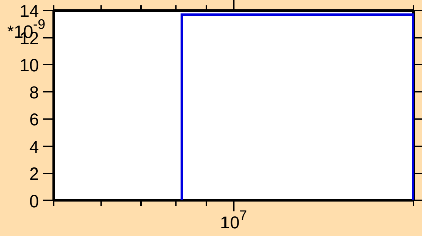
\sigma vs. E for ^{193}\text{Bi}(n,\text{pd})
