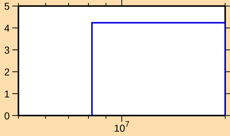
\Delta\sigma/\sigma vs. E for ^{193}\text{Bi}(n,\text{tot.})
