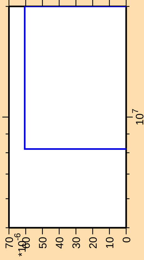
\Delta\sigma/\sigma vs. E for ^{193}\text{Bi} (mt 42)
