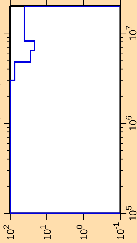
\Delta\sigma/\sigma vs. E for ^{193}\text{Bi}(n,\text{inel.})
