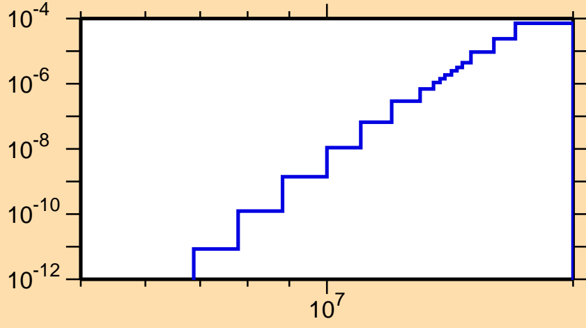
\sigma vs. E for ^{194}\text{Bi}(n,\text{He}3)
