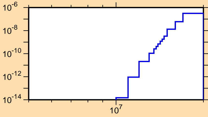
\sigma vs. E for ^{194}\text{Bi}(n,\text{pd})
