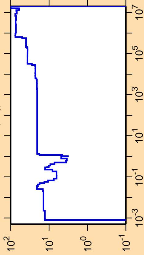
\Delta\sigma/\sigma vs. E for ^{194}\text{Bi}(n,\gamma)
