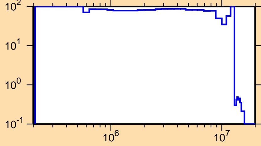
\Delta\sigma/\sigma vs. E for ^{194}\text{Bi}(n,n_1)
