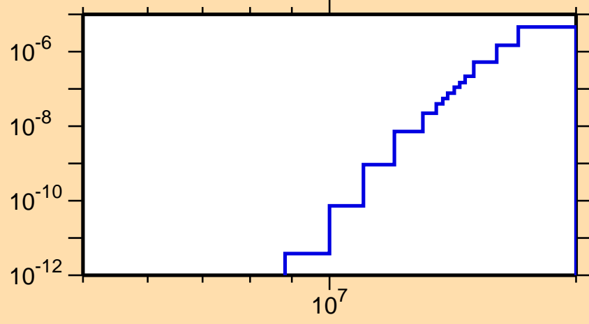
\sigma vs. E for ^{194}\text{Bi} (mt 45)
