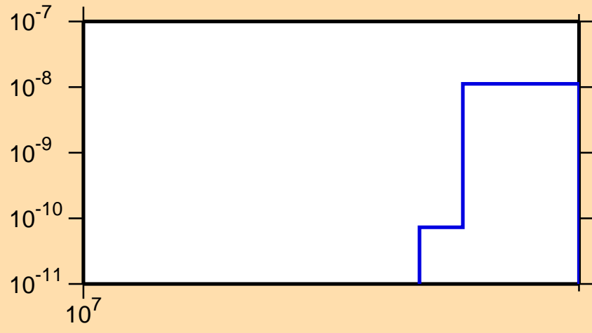
\sigma vs. E for ^{194}\text{Bi}(n,nt)
