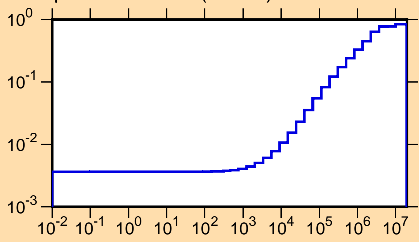
\mu vs. E for ^{194}\text{Bi}(\text{mt251})
