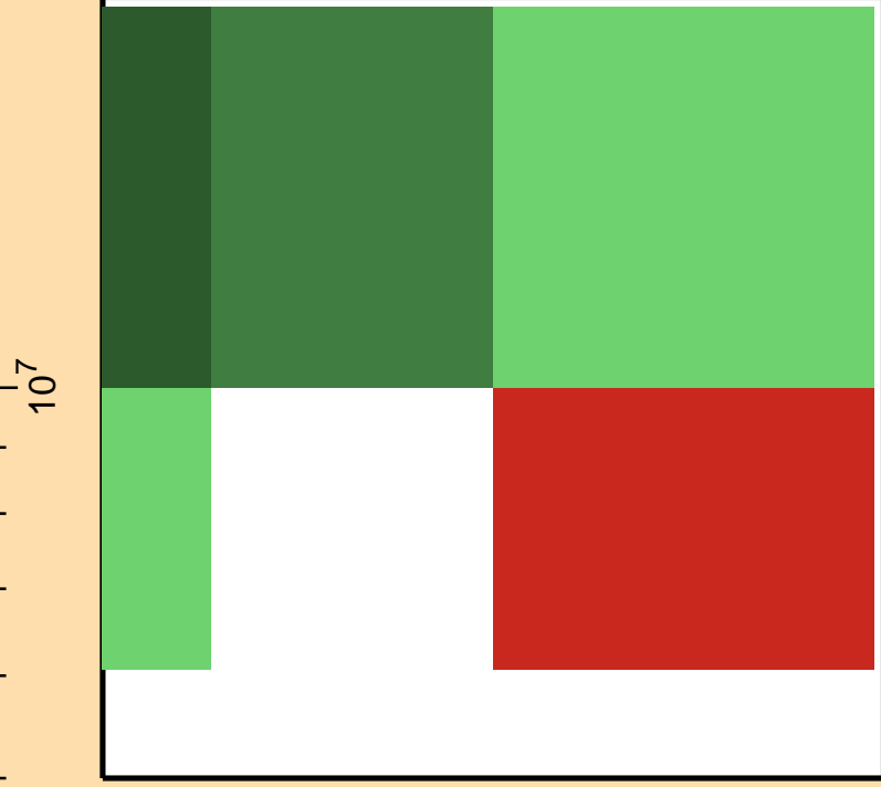
\Delta\sigma/\sigma vs. E for ^{194}\text{Bi}(n,\text{nonel.})
