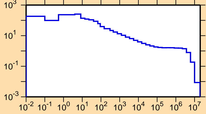
\sigma vs. E for ^{194}\text{Bi}(n,\gamma)
