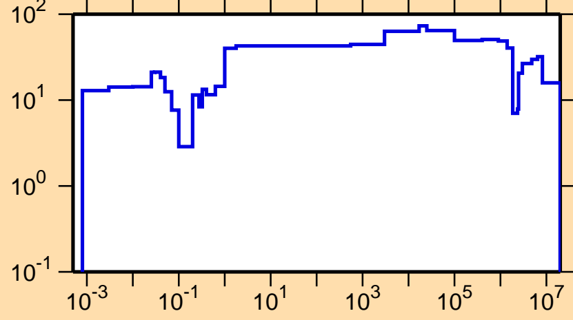
\Delta\sigma/\sigma vs. E for ^{194}\text{Bi}(n,\text{tot.})
