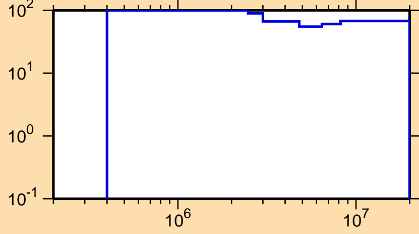
\Delta\sigma/\sigma vs. E for ^{194}\text{Bi}(n,n\text{cont.})
