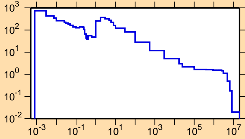
\sigma vs. E for ^{194}\text{Bi}(n,\gamma)
