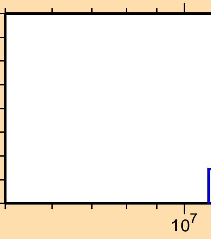
\sigma vs. E for ^{194}\text{Bi}(n,\text{nd})
