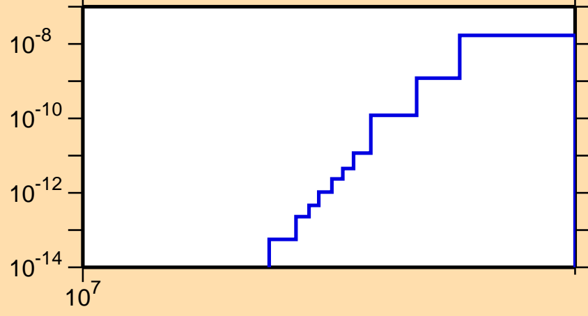
\sigma vs. E for ^{194}\text{Bi}(n,\text{pt})
