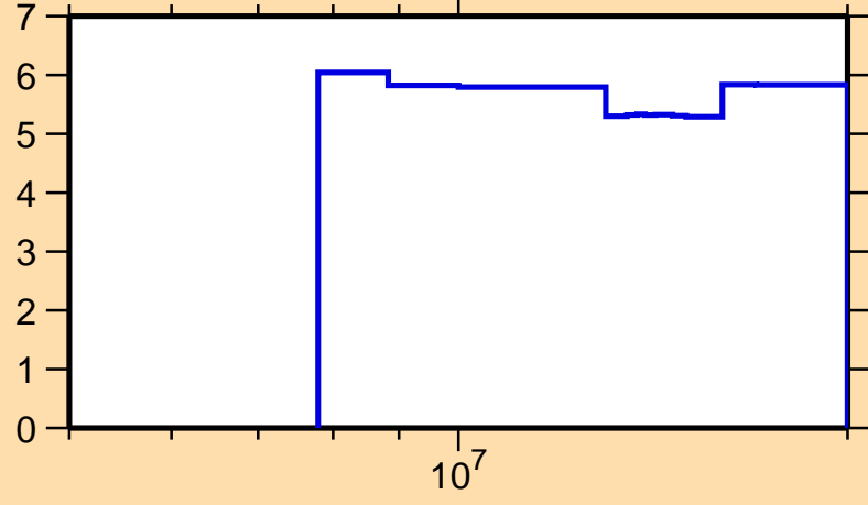
\Delta\sigma/\sigma vs. E for ^{194}\text{Bi}(n,\text{nonel.})
