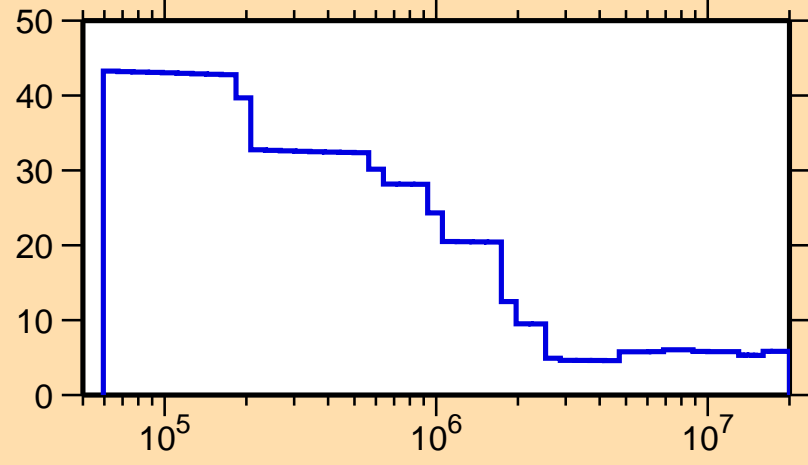
\Delta\sigma/\sigma vs. E for ^{194}\text{Bi}(n,n\text{onel.})
