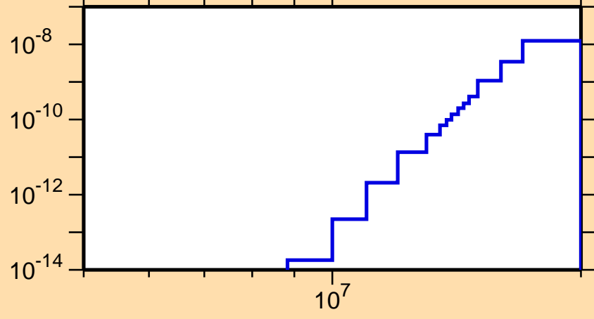
\sigma vs. E for ^{194}\text{Bi}(\text{mt117})
