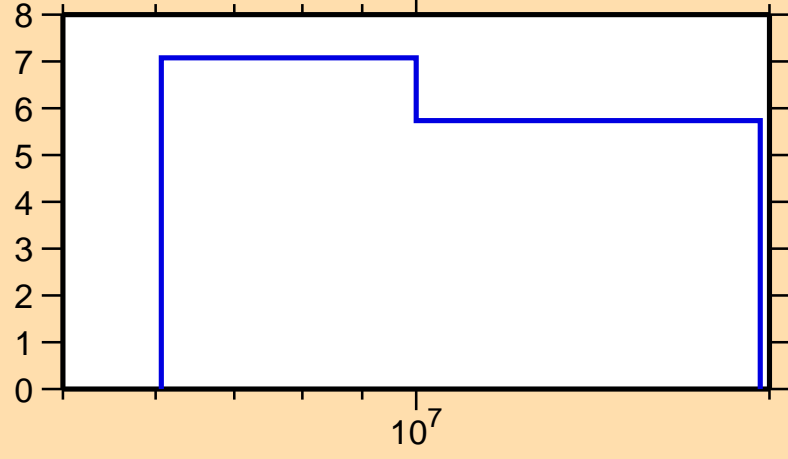
\Delta\sigma/\sigma vs. E for ^{194}\text{Bi}(n,\text{el.})
