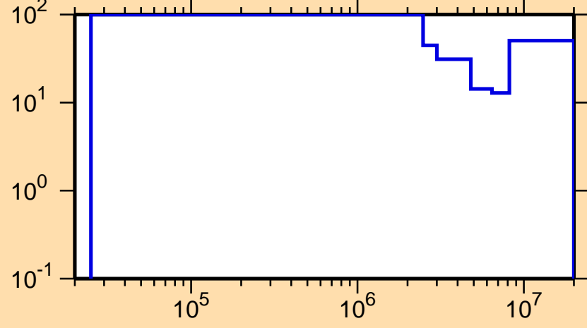
\Delta\sigma/\sigma vs. E for ^{194}\text{Bi}(n,ncont.)
