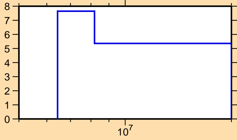
\Delta\sigma/\sigma vs. E for ^{194}\text{Bi}(n,\text{el.})
