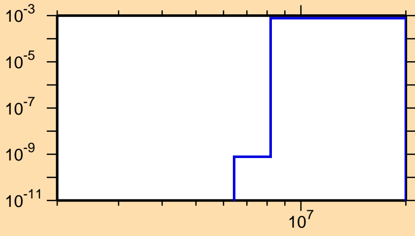
\sigma vs. E for ^{194}\text{Bi}(n,t)
