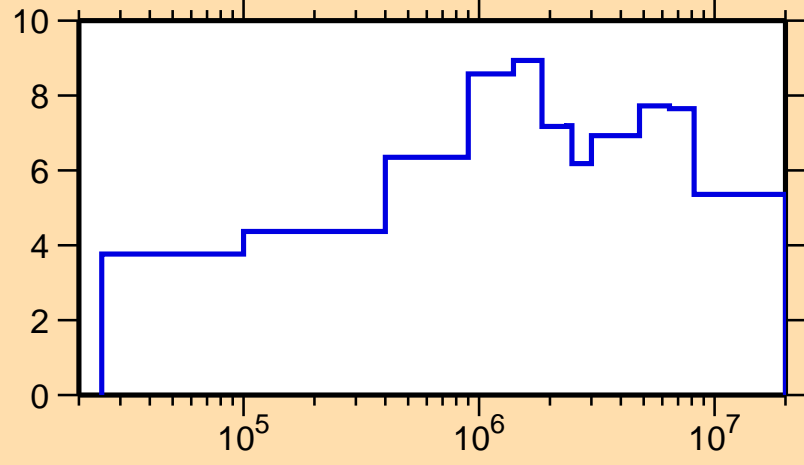
\Delta\sigma/\sigma vs. E for ^{194}\text{Bi}(n, el.)
