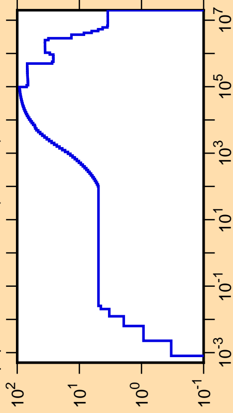
\Delta\mu/\mu vs. E for ^{195}\text{Bi}(\text{mt251})
