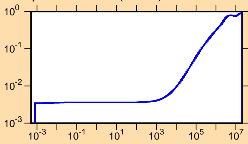
\mu vs. E for ^{195}\text{Bi}(\text{mt251})
