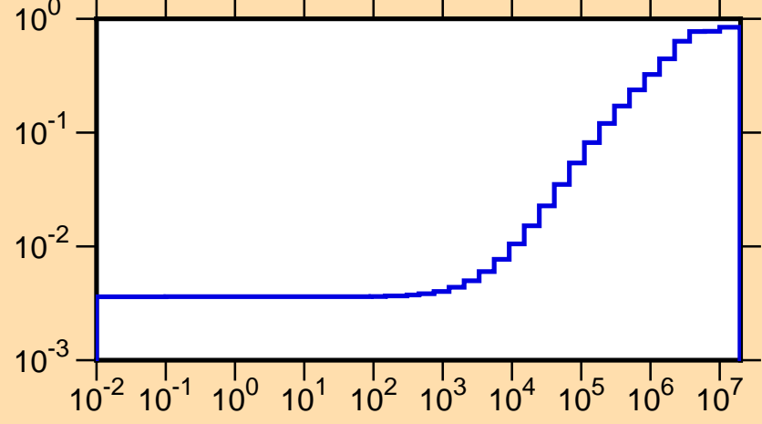
\mu vs. E for ^{195}\text{Bi}(\text{mt251})
