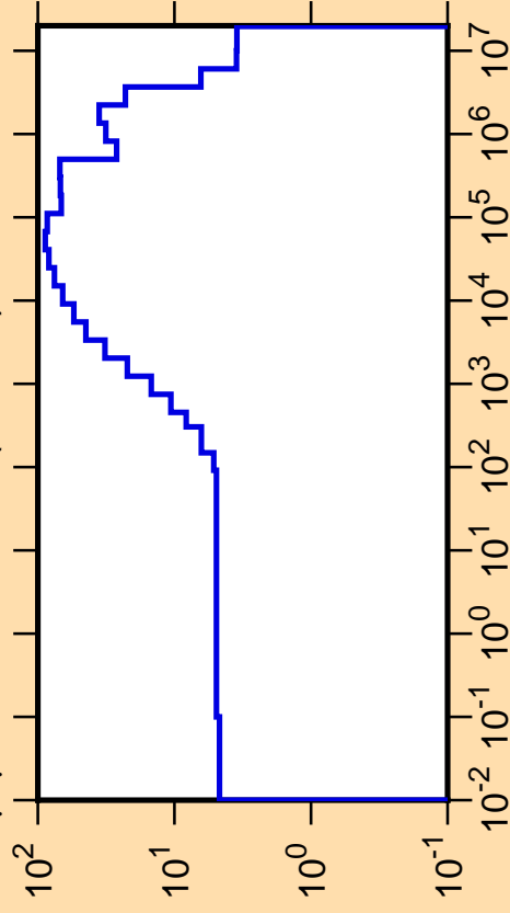
\Delta\mu/\mu vs. E for ^{195}\text{Bi}(\text{mt251})
