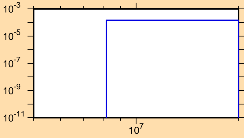
\sigma vs. E for ^{195}\text{Bi}(n,t)
