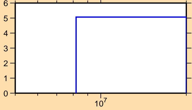
\Delta\sigma/\sigma vs. E for ^{195}\text{Bi}(n,\text{nonel.})
