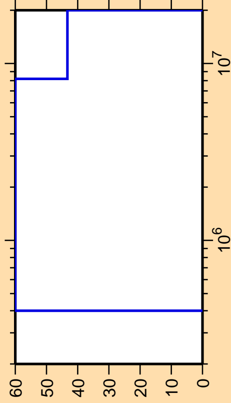
\Delta\sigma/\sigma vs. E for ^{195}\text{Bi}(n,p)
