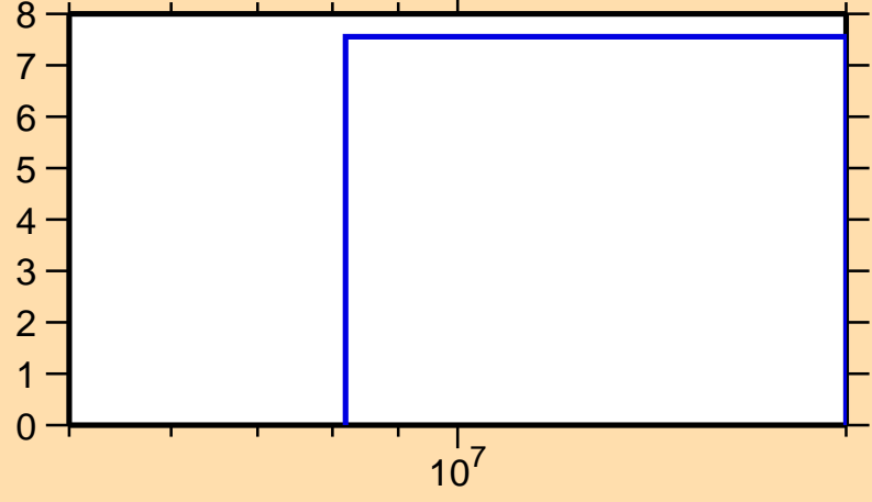
\Delta\sigma/\sigma vs. E for ^{195}\text{Bi}(n,\text{el.})
