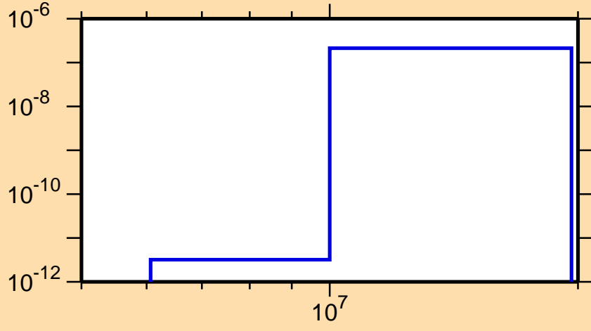
\sigma vs. E for ^{195}\text{Bi}(\text{mt } 45)
