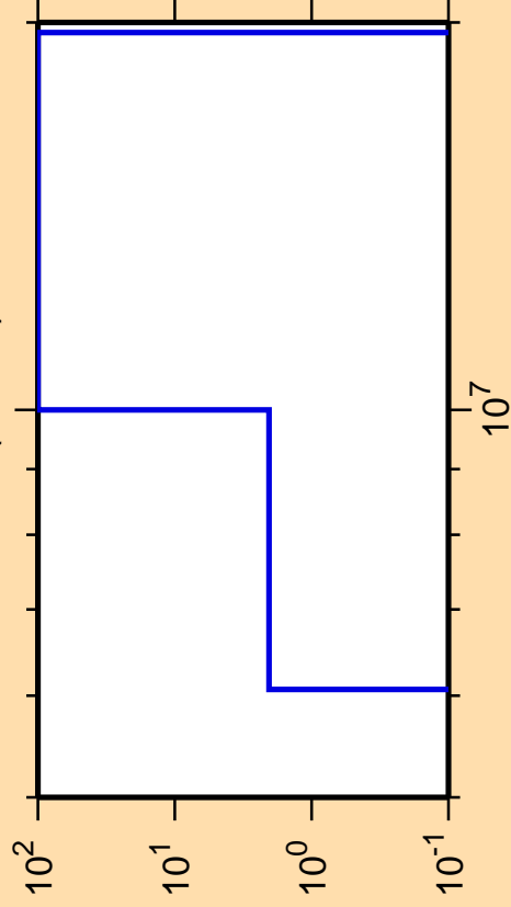
\Delta\sigma/\sigma vs. E for ^{195}\text{Bi}(\text{mt } 45)
