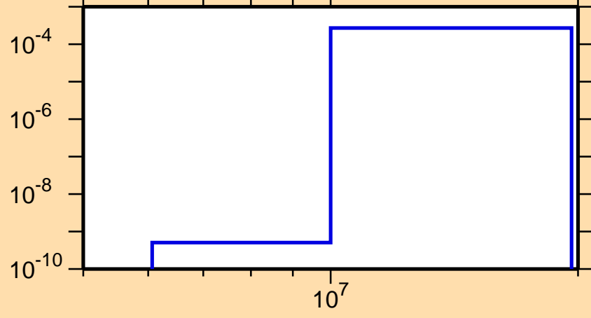
\sigma vs. E for ^{195}\text{Bi}(n,t)
