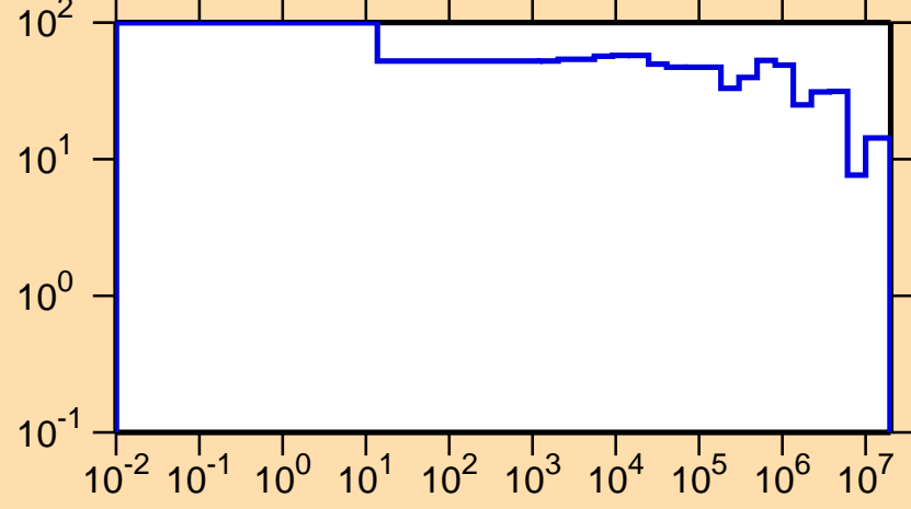
\Delta\sigma/\sigma vs. E for ^{195}\text{Bi}(n,\text{el.})
