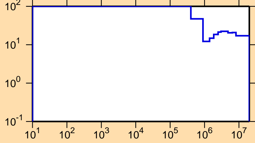
\Delta\sigma/\sigma vs. E for ^{195}\text{Bi}(n,\text{nonel.})
