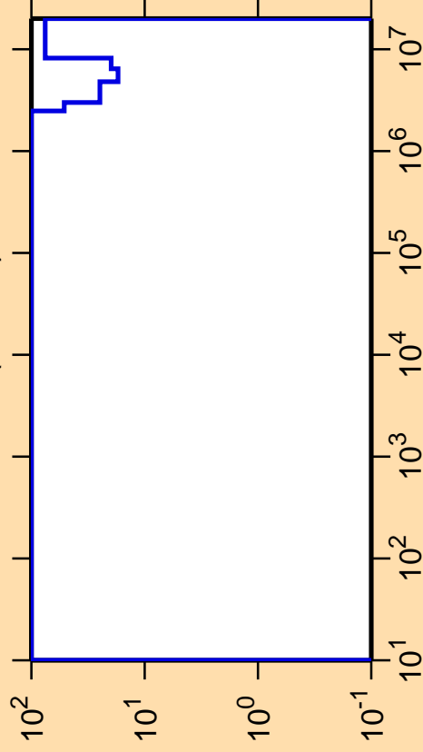
\Delta\sigma/\sigma vs. E for ^{195}\text{Bi}(n,\text{inel.})
