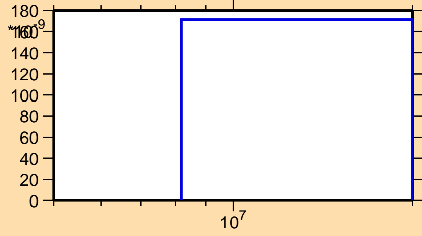
\sigma vs. E for ^{195}\text{Bi}(\text{mt } 45)
