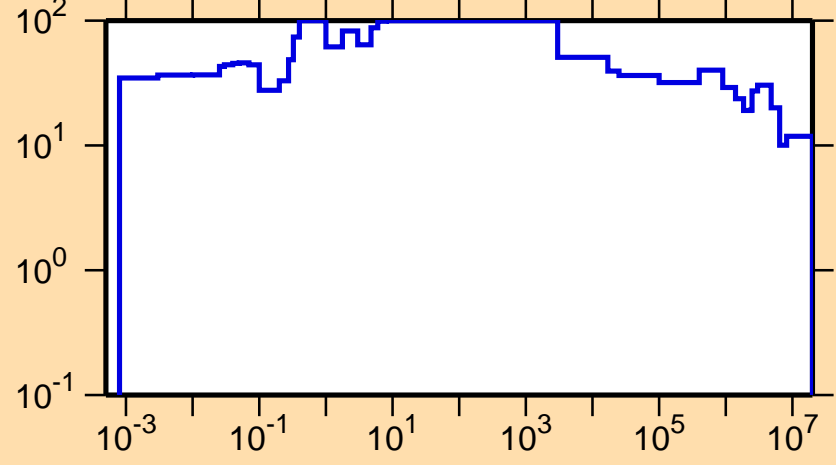
\Delta\sigma/\sigma vs. E for ^{195}\text{Bi}(n,\text{tot.})
