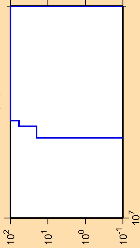
\Delta\sigma/\sigma vs. E for ^{196}\text{Bi}(n,pd)
