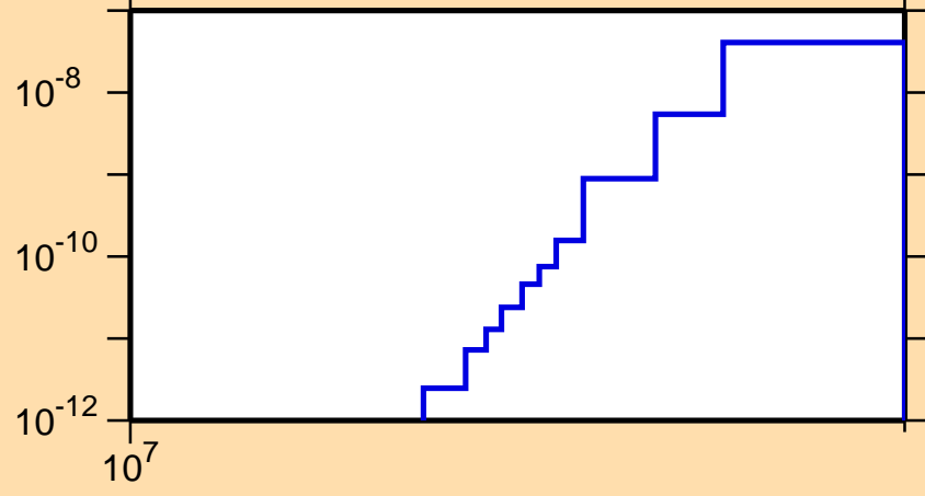
\sigma vs. E for ^{196}\text{Bi}(n,pd)
