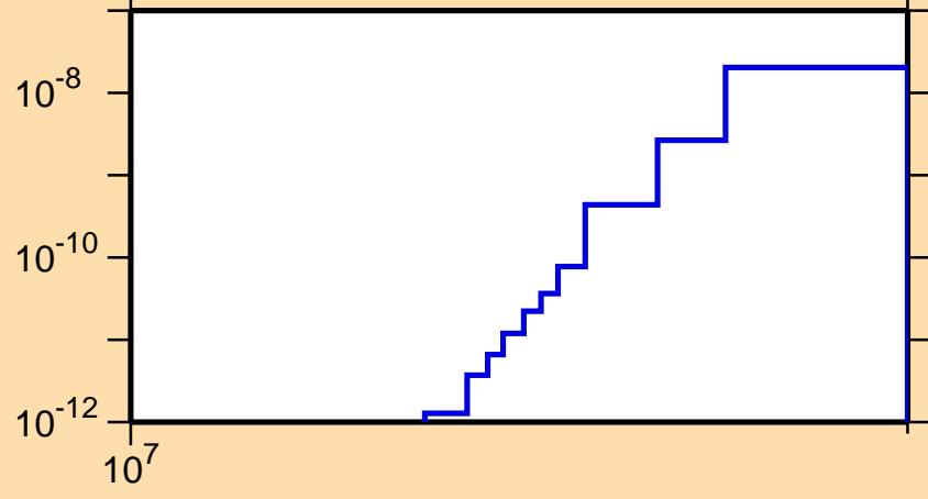
\sigma vs. E for ^{196}\text{Bi}(n,\text{pd})
