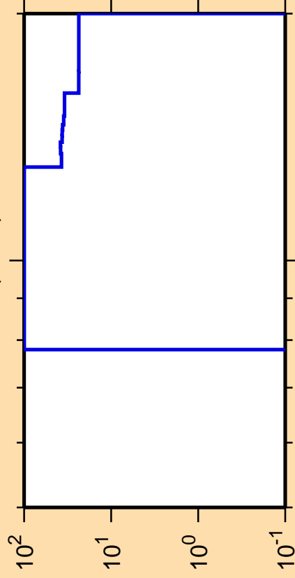
\Delta\sigma/\sigma vs. E for ^{196}\text{Bi}(n,2n)
