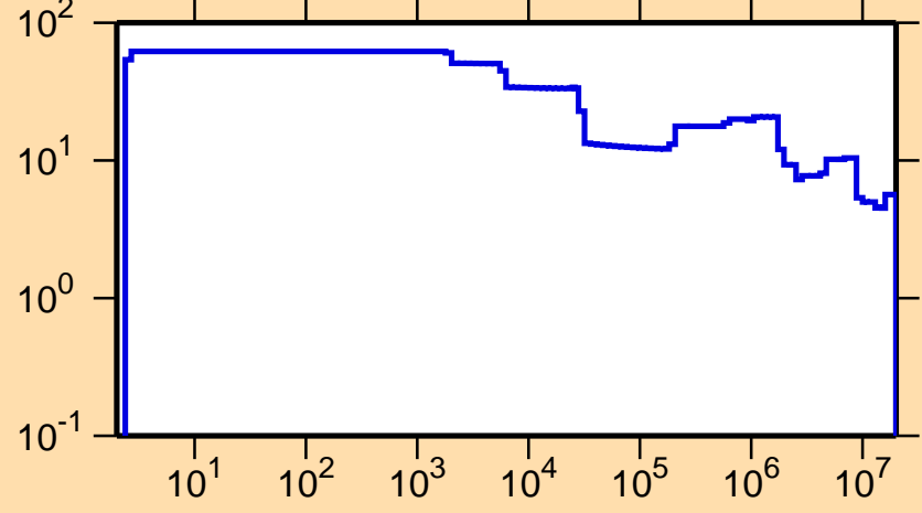
\Delta\sigma/\sigma vs. E for ^{196}\text{Bi}(n,\text{tot.})
