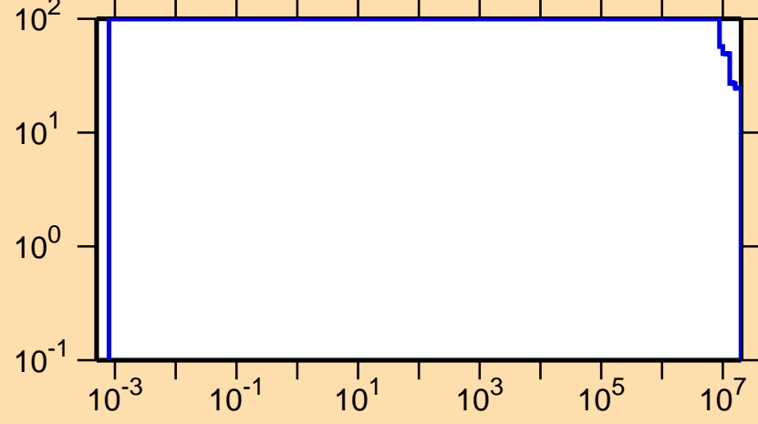
\Delta\sigma/\sigma vs. E for ^{196}\text{Bi}(n,p)
