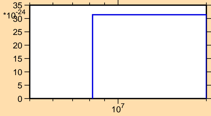
\sigma vs. E for ^{196}\text{Bi} (mt 42)
