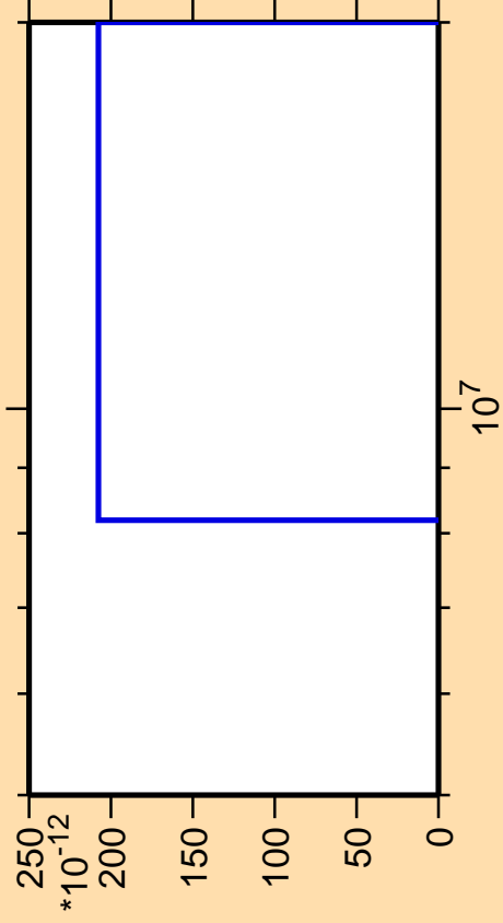
\Delta\sigma/\sigma vs. E for ^{196}\text{Bi} (mt 42)
