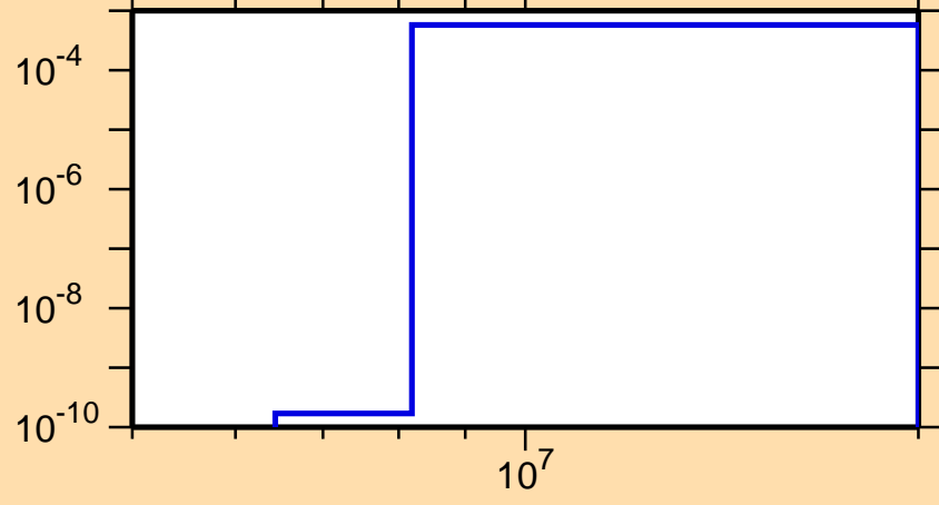
\sigma vs. E for ^{196}\text{Bi}(n,t)
