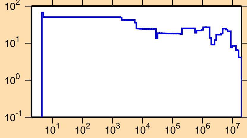
\Delta\sigma/\sigma vs. E for ^{198}\text{Bi}(n,\text{el.})
