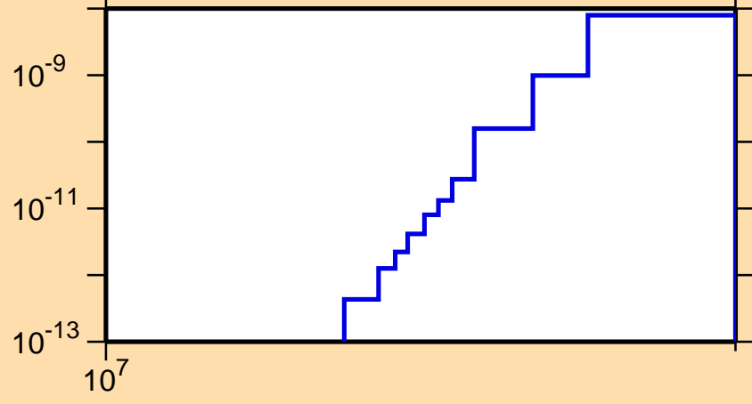
\sigma vs. E for ^{198}\text{Bi}(n,\text{pd})
