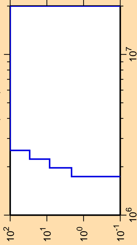
\Delta\sigma/\sigma vs. E for ^{198}\text{Bi}(n,n\alpha)
