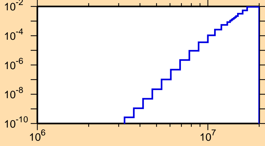
\sigma vs. E for ^{198}\text{Bi}(n,n\alpha)
