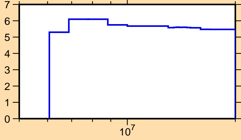
\Delta\sigma/\sigma vs. E for ^{198}\text{Bi}(n,\text{nonel.})
