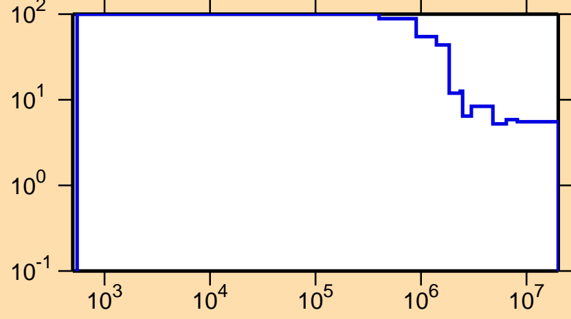
\Delta\sigma/\sigma vs. E for ^{198}\text{Bi}(n,n\text{onel.})
