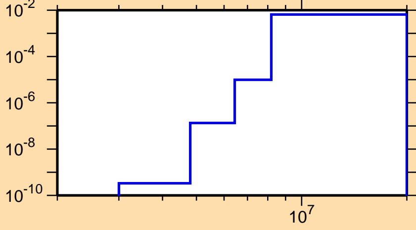
\sigma vs. E for ^{198}\text{Bi}(n,d)
