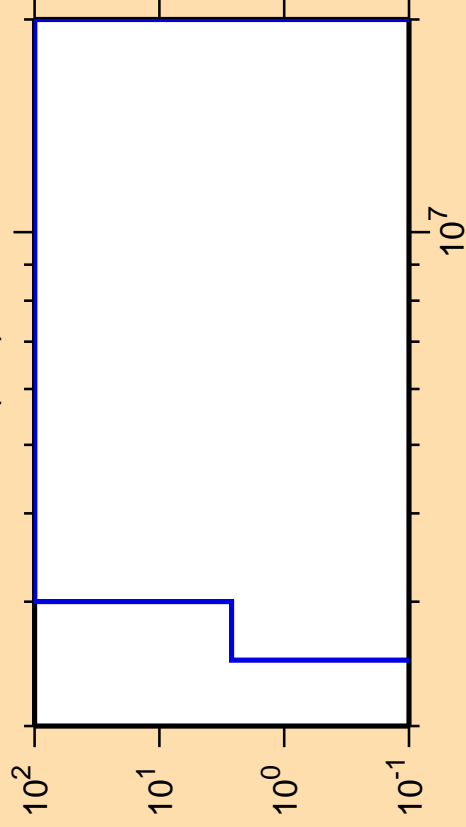
\Delta\sigma/\sigma vs. E for ^{198}\text{Bi}(n,d)
