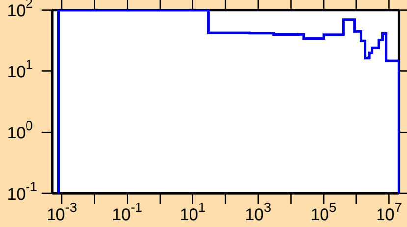
\Delta\sigma/\sigma vs. E for ^{199}\text{Bi}(n,\text{el.})
