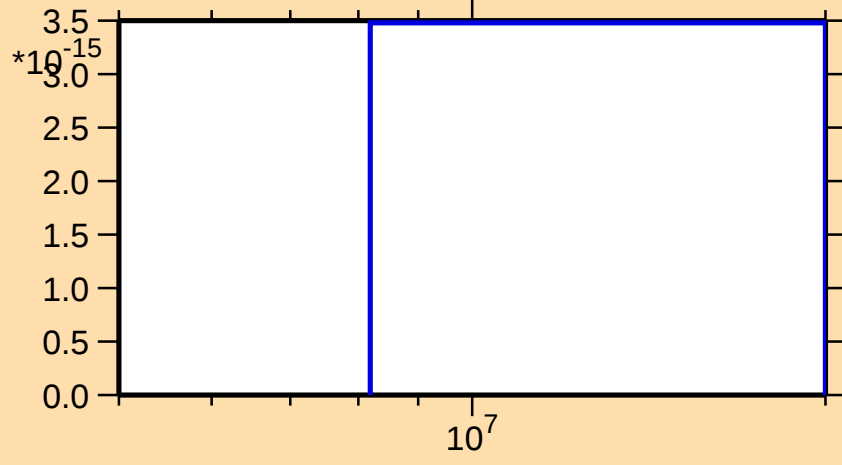
\sigma vs. E for ^{199}\text{Bi}(\text{mt } 34)
