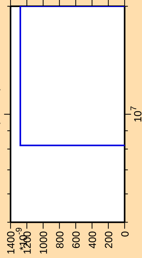
\Delta\sigma/\sigma vs. E for ^{199}\text{Bi}(\text{mt } 42)
