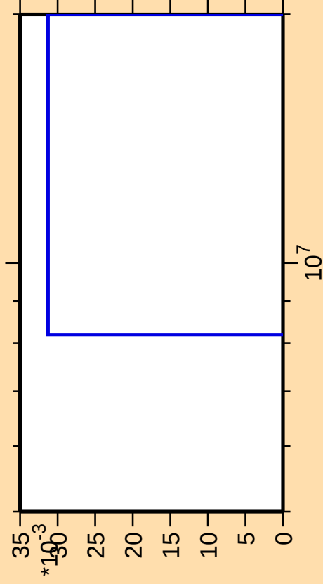
\Delta\sigma/\sigma vs. E for ^{199}\text{Bi}(\text{mt } 34)
