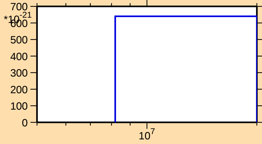
\sigma vs. E for ^{199}\text{Bi}(\text{mt } 42)
