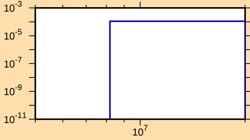
\sigma vs. E for ^{199}\text{Bi}(n,t)
