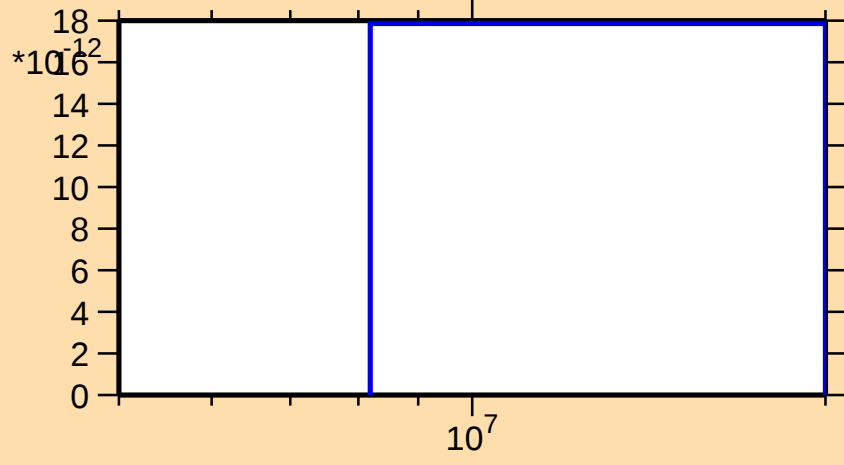
\sigma vs. E for ^{199}\text{Bi}(\text{mt } 45)
