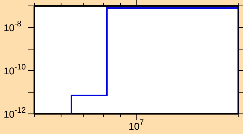
\sigma vs. E for ^{199}\text{Bi}(n,p\alpha)
