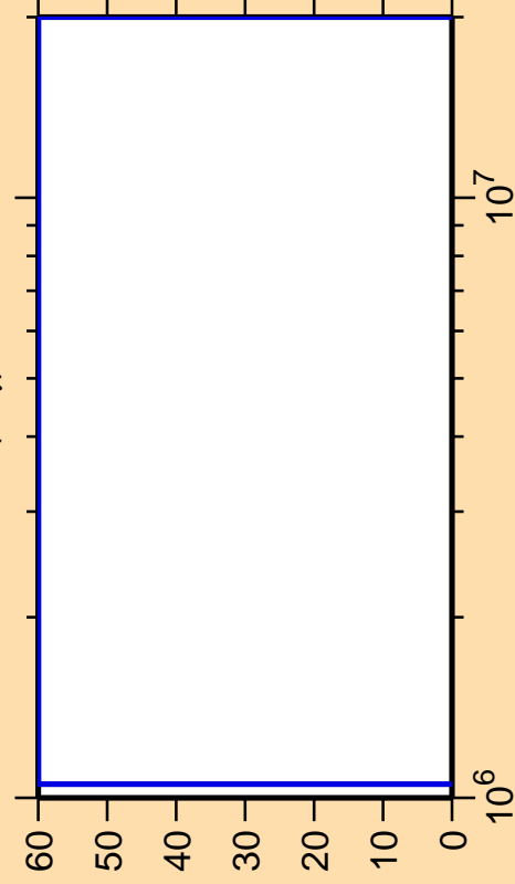
\Delta\sigma/\sigma vs. E for ^{199}\text{Bi}(n,\gamma)
