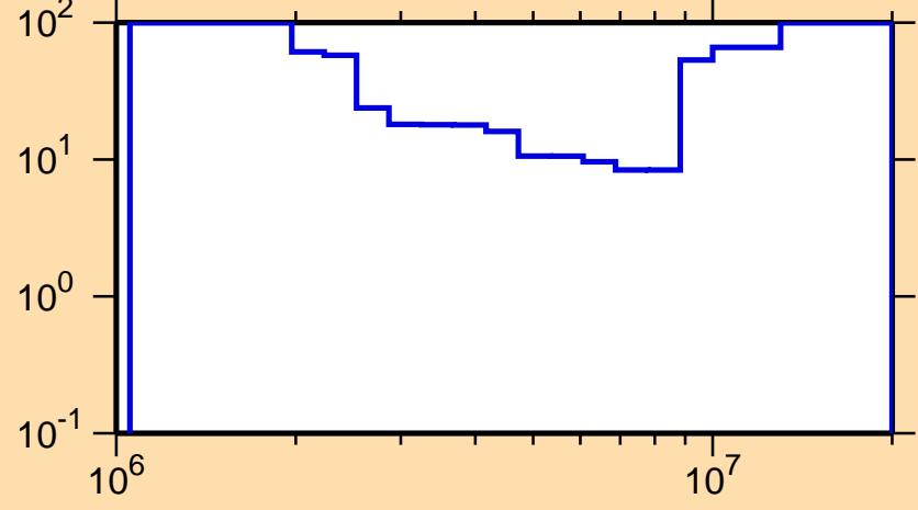
\Delta\sigma/\sigma vs. E for ^{199}\text{Bi}(n,n\text{cont.})
