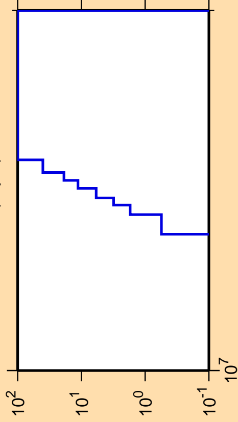
\Delta\sigma/\sigma vs. E for ^{199}\text{Bi}(n,pd)
