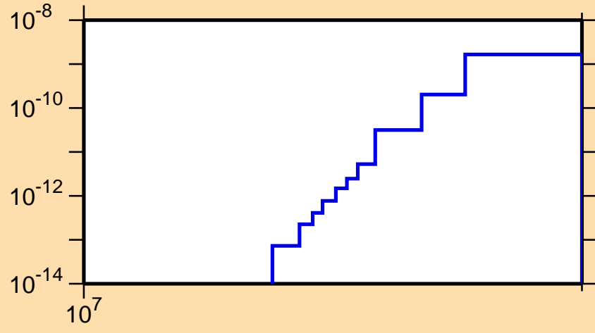
\sigma vs. E for ^{199}\text{Bi}(n,pd)
