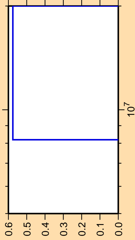
\Delta\sigma/\sigma vs. E for ^{199}\text{Bi}(\text{mt } 34)
