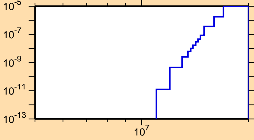
\sigma vs. E for ^{200}\text{Bi}(n,\text{nd})
