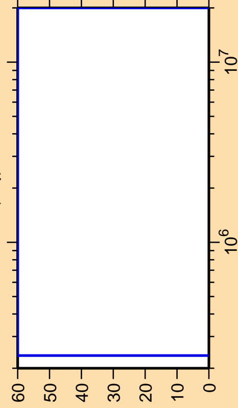
\Delta\sigma/\sigma vs. E for ^{200}\text{Bi}(n,\gamma)
