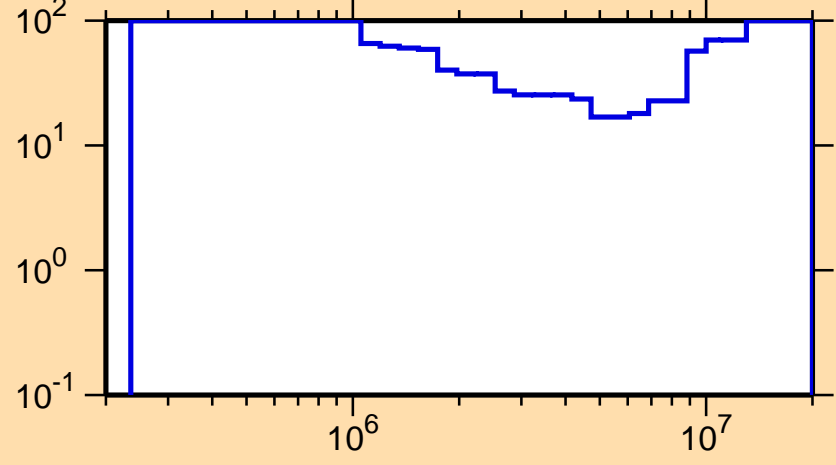
\Delta\sigma/\sigma vs. E for ^{200}\text{Bi}(n,n\text{cont.})
