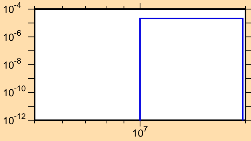
\sigma vs. E for ^{200}\text{Bi}(n,2np)
