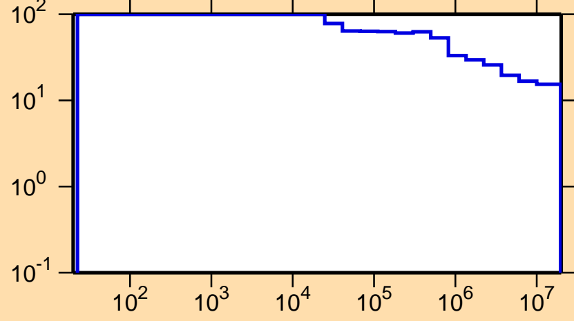
\Delta\sigma/\sigma vs. E for ^{200}\text{Bi}(n,\text{nonel.})
