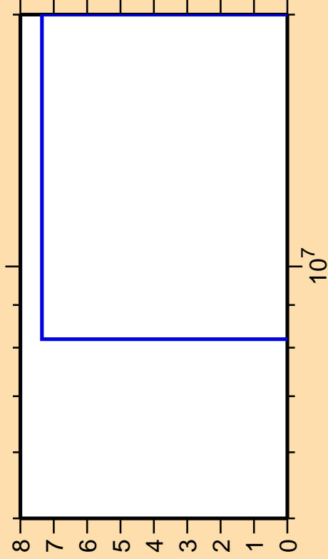
\Delta\sigma/\sigma vs. E for ^{200}\text{Bi}(\text{mt } 45)
