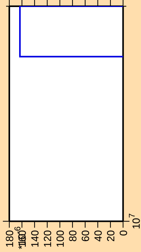
\Delta\sigma/\sigma vs. E for ^{201}\text{Bi}(\text{mt } 42)
