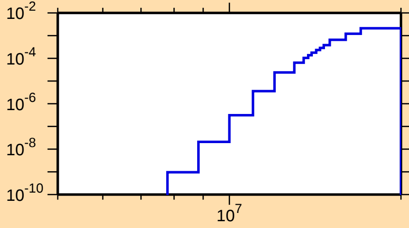
\sigma vs. E for ^{201}\text{Bi}(n,t)
