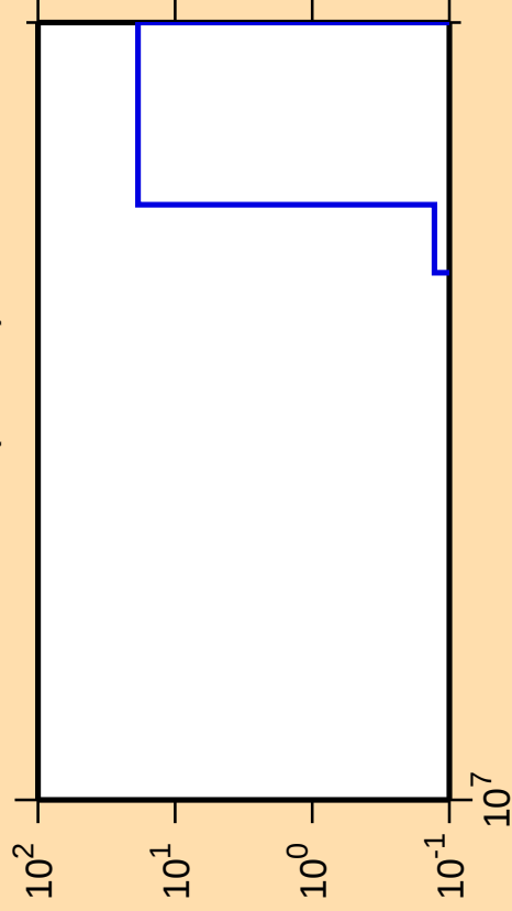
\Delta\sigma/\sigma vs. E for ^{201}\text{Bi}(\text{mt } 34)
