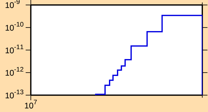
\sigma vs. E for ^{201}\text{Bi}(\text{mt } 45)
