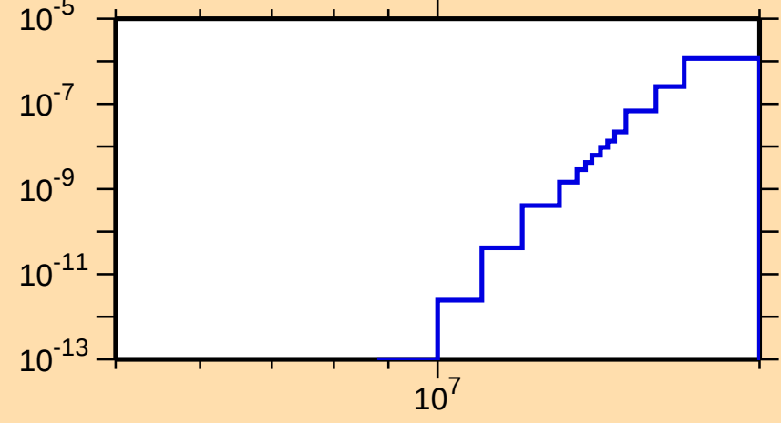
\sigma vs. E for ^{201}\text{Bi}(n,\text{He3})
