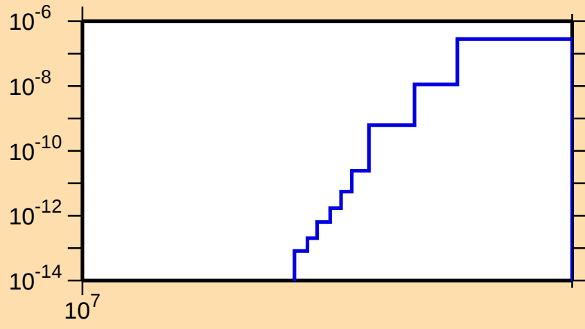
\sigma vs. E for ^{201}\text{Bi}(n,\text{nt})
