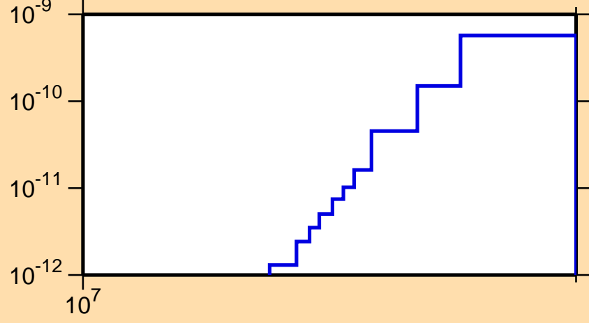
\sigma vs. E for ^{205}\text{Bi}(n,p\alpha)
