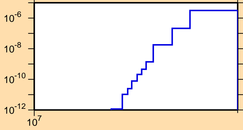
\sigma vs. E for ^{205}\text{Bi}(n,\text{nd})
