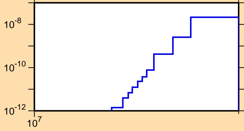
\sigma vs. E for ^{205}\text{Bi}(n,\text{He3})
