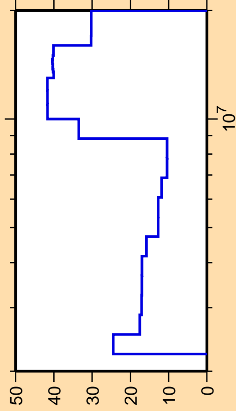
\Delta\sigma/\sigma vs. E for ^{205}\text{Bi}(n,\text{ncont.})
