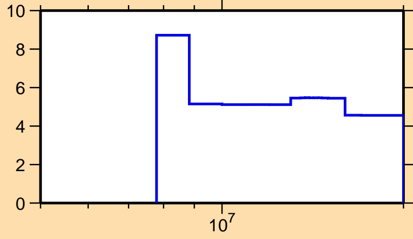
\Delta\sigma/\sigma vs. E for ^{205}\text{Bi}(n,\text{tot.})
