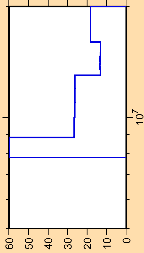
\Delta\sigma/\sigma vs. E for ^{205}\text{Bi}(n,2n)
