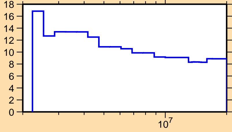
\Delta\sigma/\sigma vs. E for ^{205}\text{Bi}(n,n\text{onel.})
