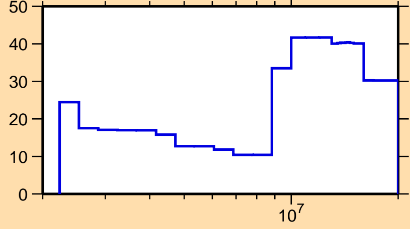
\Delta\sigma/\sigma vs. E for ^{205}\text{Bi}(n,n\text{cont.})
