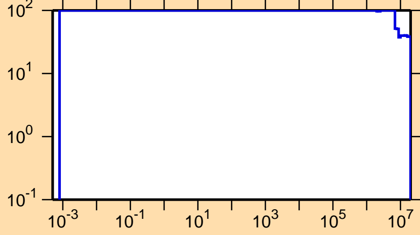
\Delta\sigma/\sigma vs. E for ^{205}\text{Bi}(n,p)
