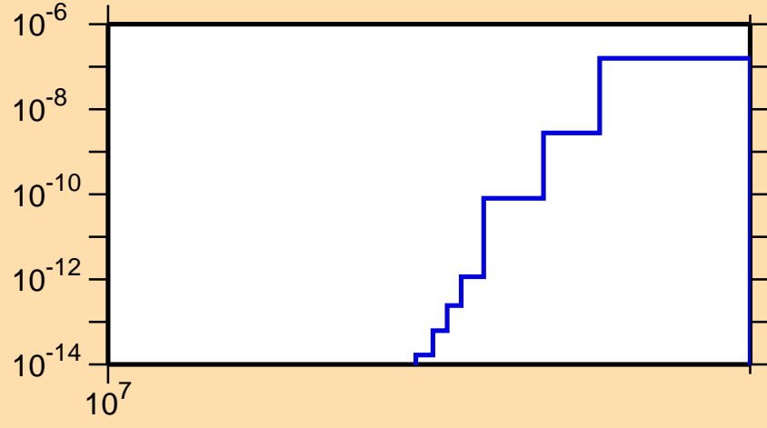
\sigma vs. E for ^{205}\text{Bi}(n,nt)
