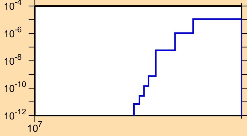
\sigma vs. E for ^{205}\text{Bi}(n,2np)
