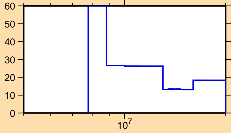
\Delta\sigma/\sigma vs. E for ^{205}\text{Bi}(n,2n)
