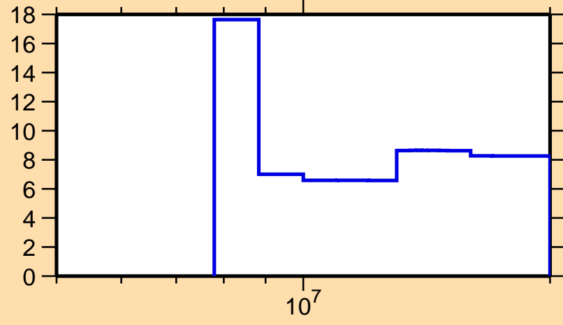
\Delta\sigma/\sigma vs. E for ^{205}\text{Bi}(n,\text{el.})
