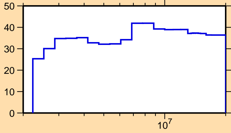
\Delta\sigma/\sigma vs. E for ^{205}\text{Bi}(n,n_1)
