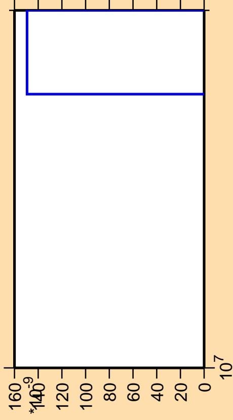
\Delta\sigma/\sigma vs. E for ^{205}\text{Bi} (mt 42)
