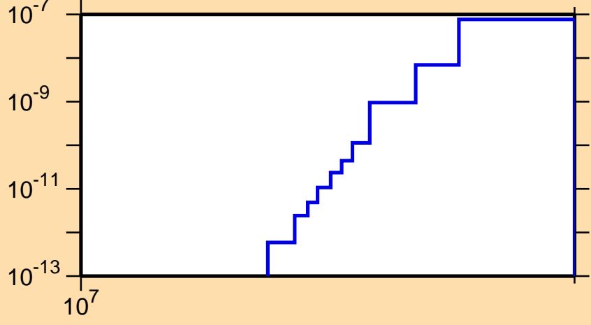
\sigma vs. E for ^{205}\text{Bi}(n,2n\alpha)
