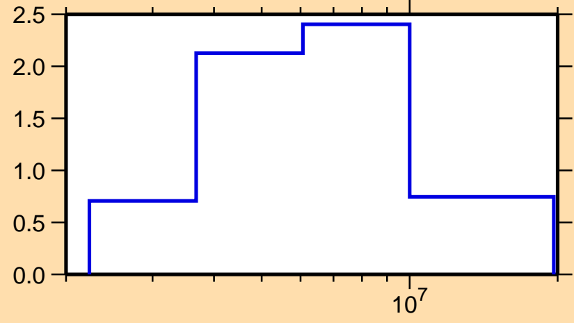
\sigma vs. E for ^{205}\text{Bi}(n,n\text{cont.})
