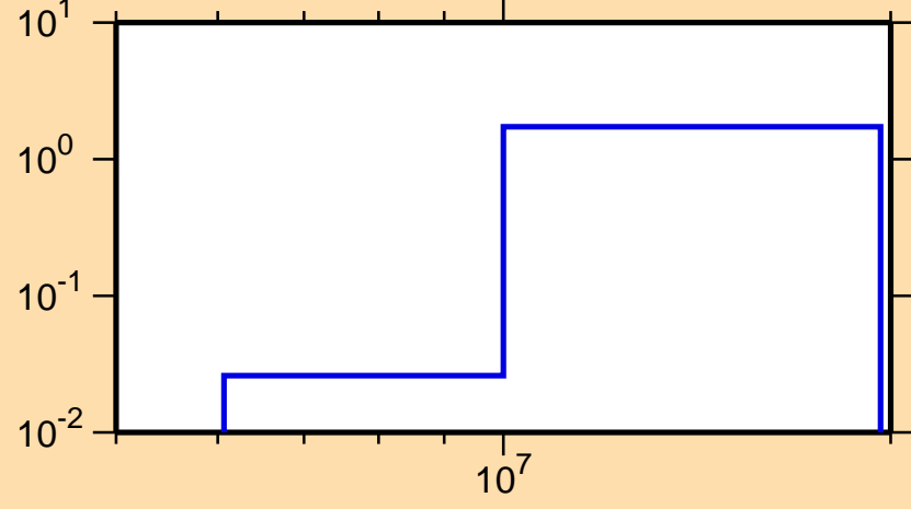
\sigma vs. E for ^{205}\text{Bi}(n,2n)
