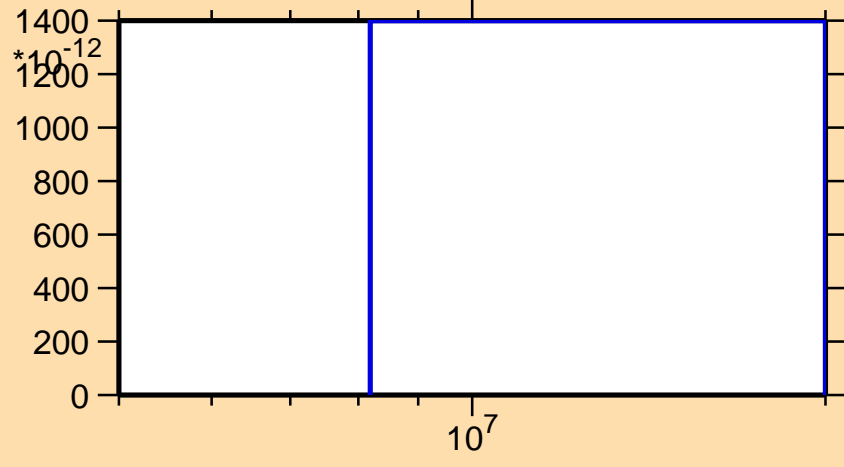
\sigma vs. E for ^{205}\text{Bi}(n,\text{nt})
