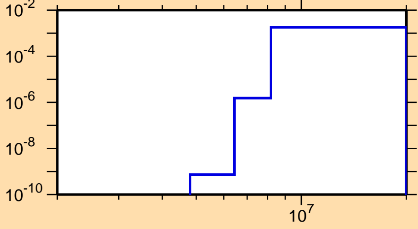
\sigma vs. E for ^{205}\text{Bi}(n,np)
