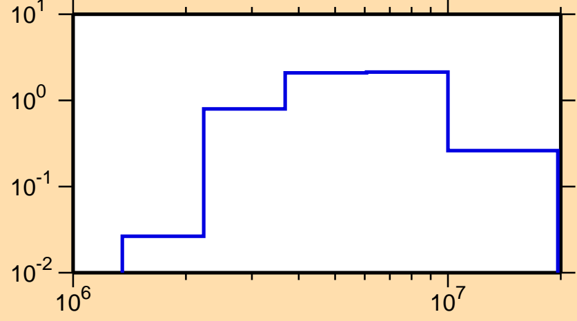
\sigma vs. E for ^{208}\text{Bi}(n,n\text{cont.})
