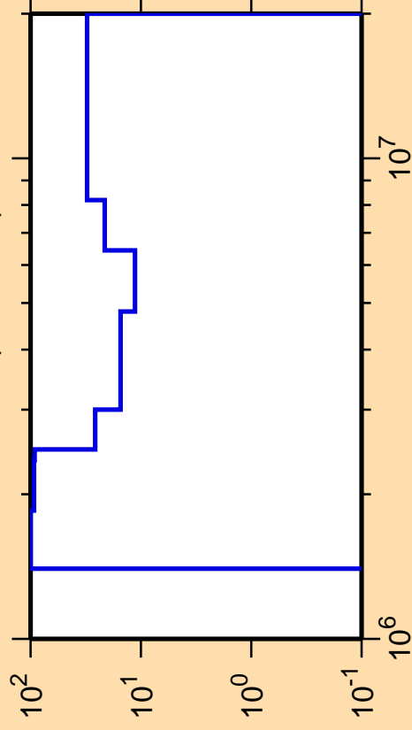
\Delta\sigma/\sigma vs. E for ^{208}\text{Bi}(n,\text{ncont.})
