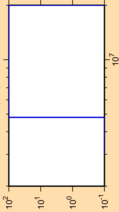
\Delta\sigma/\sigma vs. E for ^{208}\text{Bi}(n,d)
