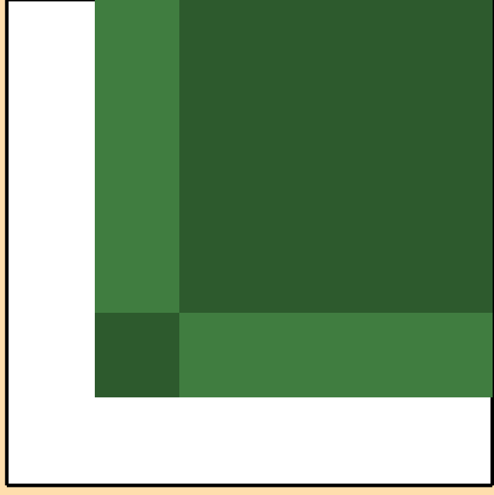
\sigma vs. E for ^{208}\text{Bi}(n,2n)
