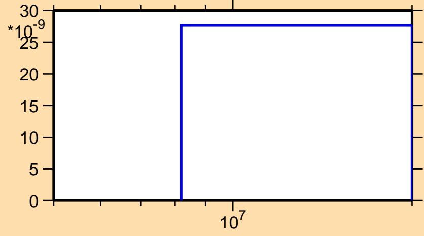
\sigma vs. E for ^{208}\text{Bi}(n,2n\alpha)
