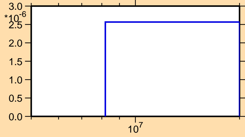
\sigma vs. E for ^{208}\text{Bi}(n,2np)
