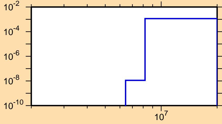
\sigma vs. E for ^{208}\text{Bi}(n,d)
