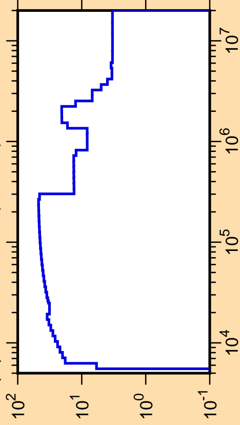
\Delta\mu/\mu vs. E for ^{209}\text{Bi}(\text{mt251})
