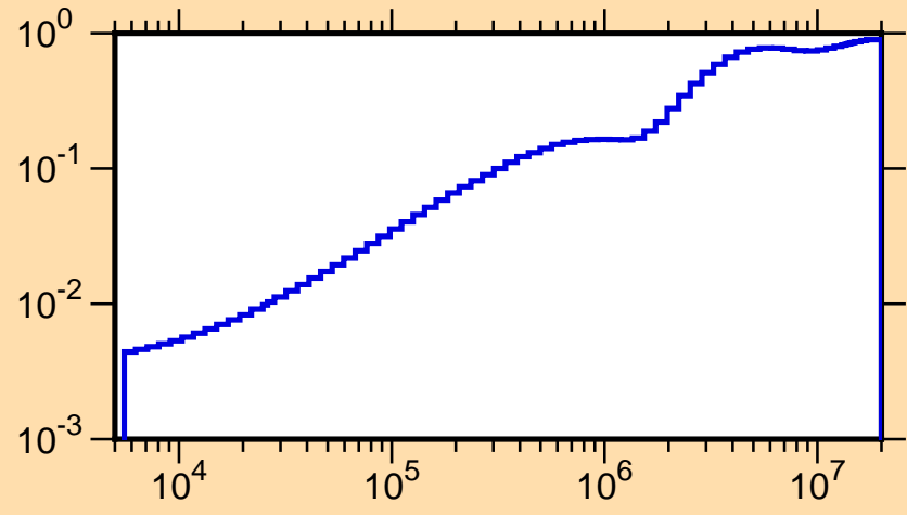
\mu vs. E for ^{209}\text{Bi}(\text{mt251})
