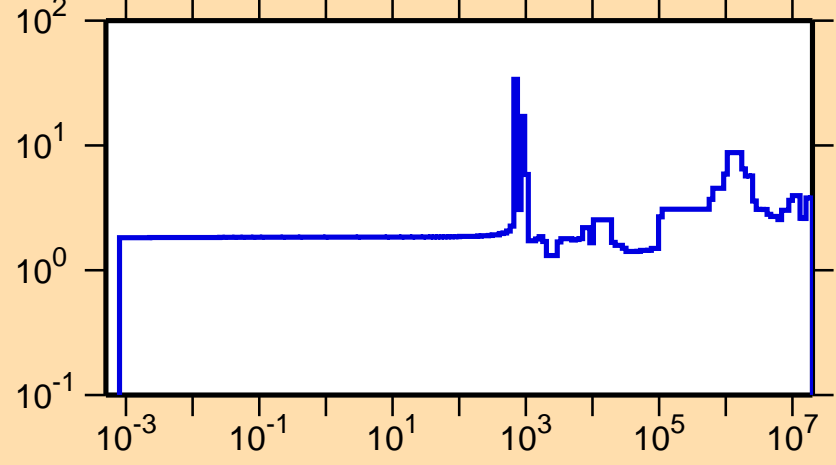
\Delta\sigma/\sigma vs. E for ^{209}\text{Bi}(n,\text{tot.})
