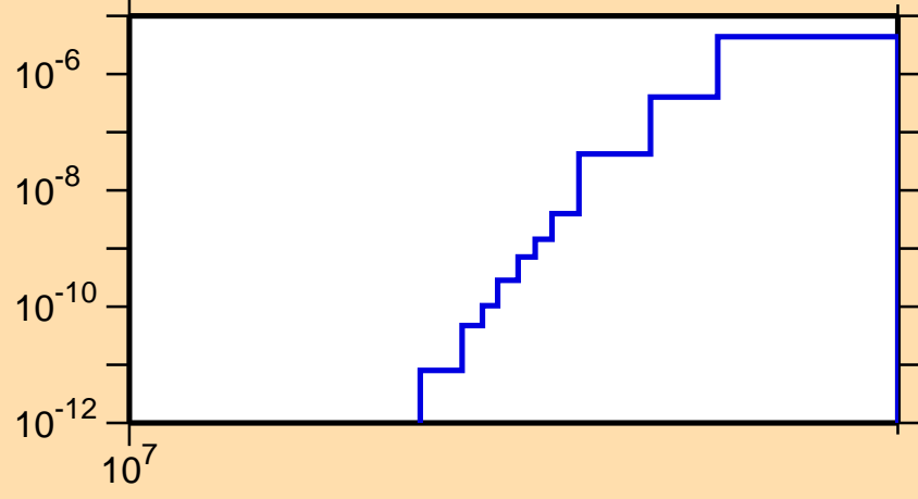
\sigma vs. E for ^{209}\text{Bi}(n,\text{nd})
