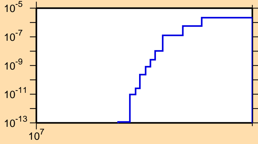
\sigma vs. E for ^{209}\text{Bi}(n,2np)
