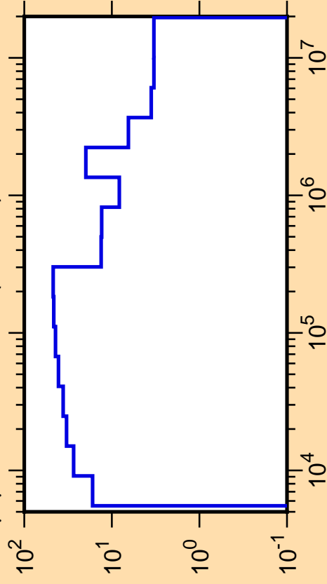
\Delta\mu/\mu vs. E for ^{209}\text{Bi}(\text{mt251})
