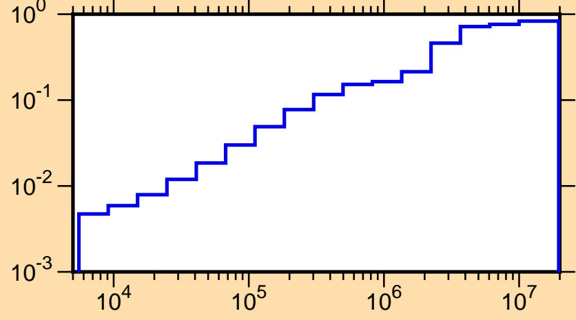
\mu vs. E for ^{209}\text{Bi}(\text{mt251})
