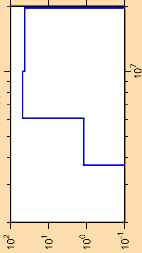
\Delta\sigma/\sigma vs. E for ^{209}\text{Bi}(n,np)
