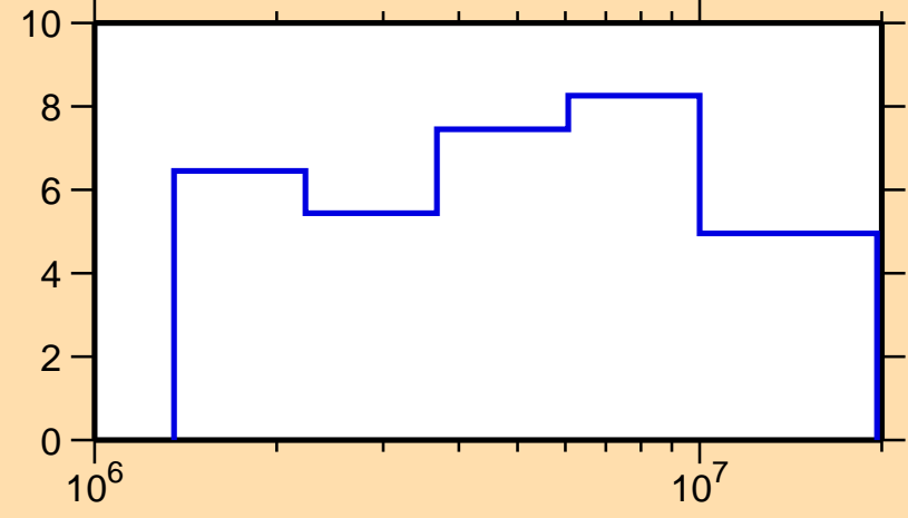
\Delta\sigma/\sigma vs. E for ^{209}\text{Bi}(n,el.)
