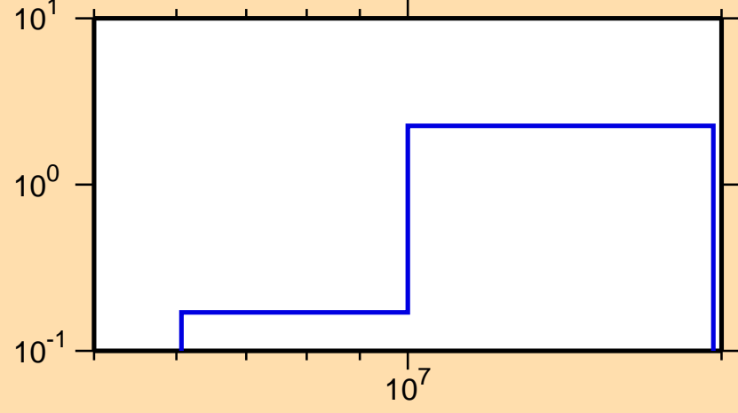
\sigma vs. E for ^{209}\text{Bi}(n,2n)
