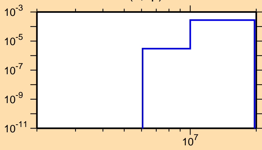
\sigma vs. E for ^{209}\text{Bi}(n,np)
