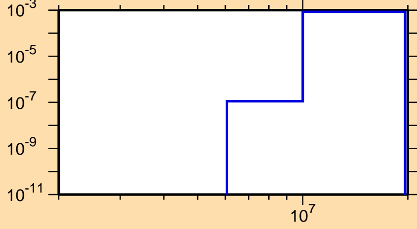
\sigma vs. E for ^{209}\text{Bi}(n,d)
