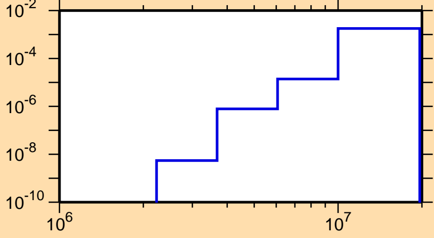
\sigma vs. E for ^{209}\text{Bi}(n,p)
