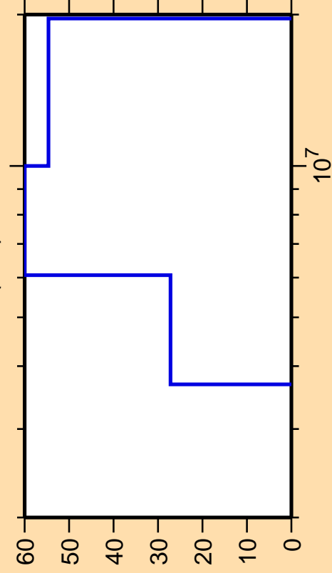
\Delta\sigma/\sigma vs. E for ^{209}\text{Bi}(n,d)
