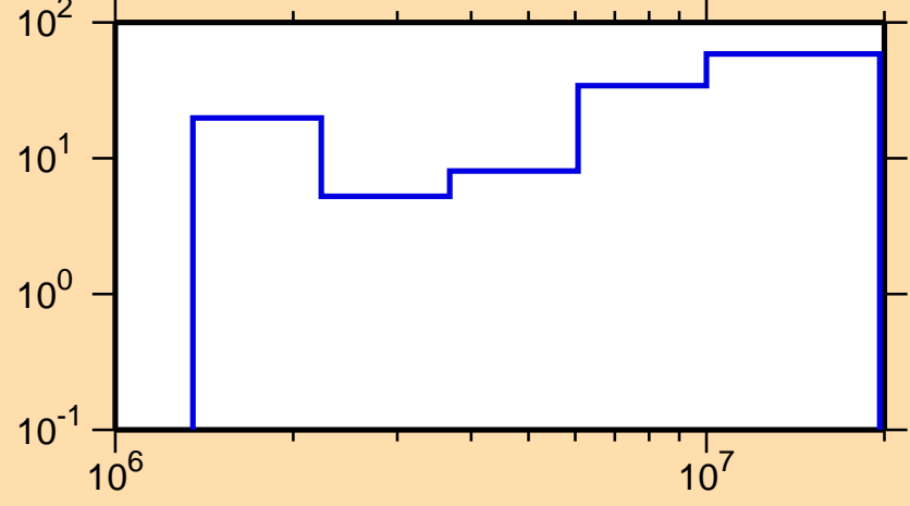
\Delta\sigma/\sigma vs. E for ^{209}\text{Bi}(n,n_1)
