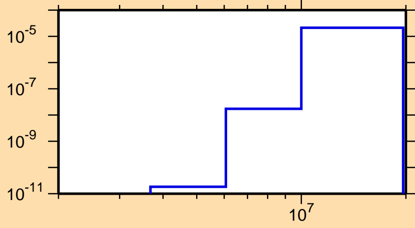
\sigma vs. E for ^{209}\text{Bi}(n,\alpha)
