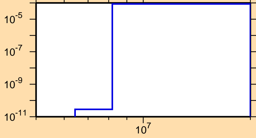
\sigma vs. E for ^{209}\text{Bi}(n,t)
