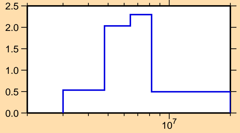
\sigma vs. E for ^{209}\text{Bi}(n,n\text{cont.})
