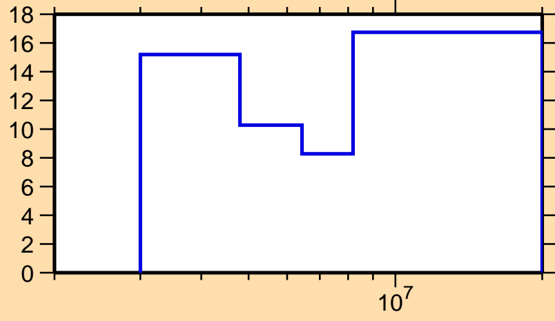
\Delta\sigma/\sigma vs. E for ^{209}\text{Bi}(n,n\text{cont.})
