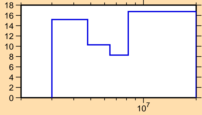
\Delta\sigma/\sigma vs. E for ^{209}\text{Bi}(n,ncont.)
