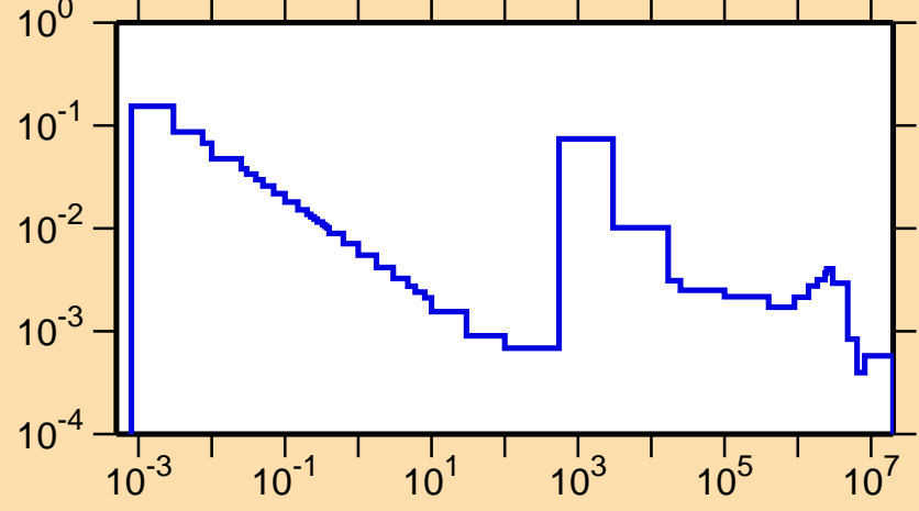
\sigma vs. E for ^{209}\text{Bi}(n,\gamma)
