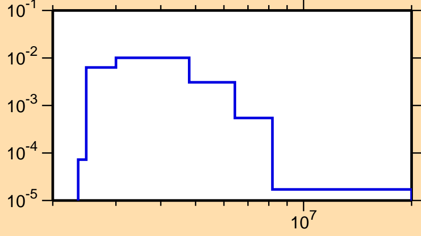
\sigma vs. E for ^{209}\text{Bi}(n,n_3)
