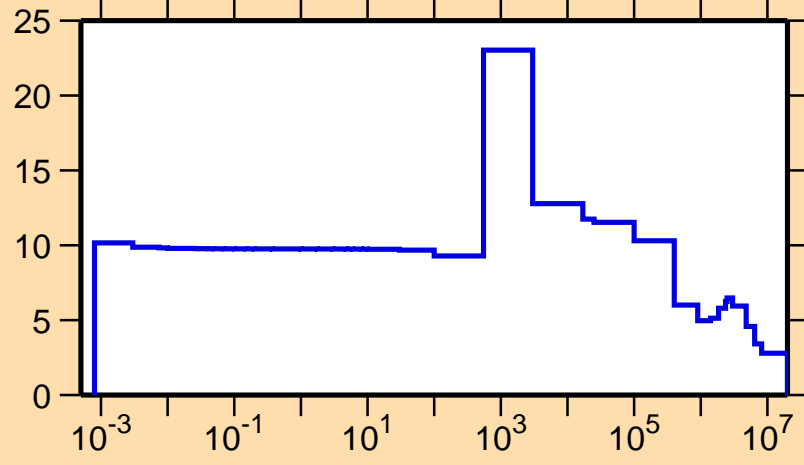
\sigma vs. E for ^{209}\text{Bi}(n,\text{el.})
