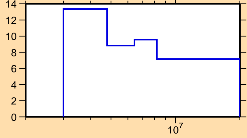
\Delta\sigma/\sigma vs. E for ^{209}\text{Bi}(n,n\text{onel.})
