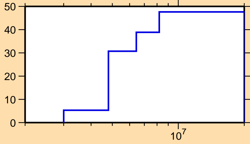
\Delta\sigma/\sigma vs. E for ^{209}\text{Bi}(n, n_1)
