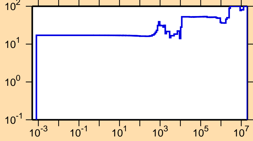
\Delta\sigma/\sigma vs. E for ^{210}\text{Bi}(n,\gamma)
