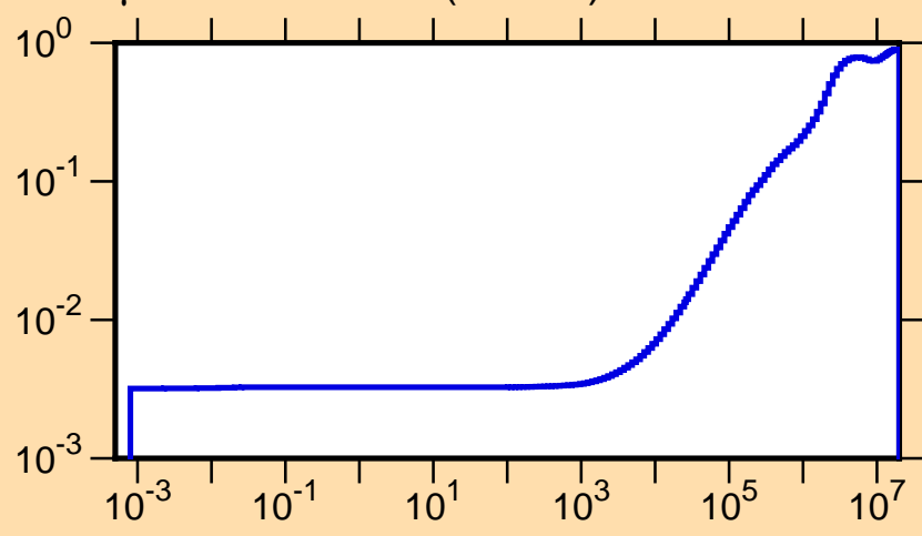
\mu vs. E for ^{211}\text{Bi}(\text{mt251})
