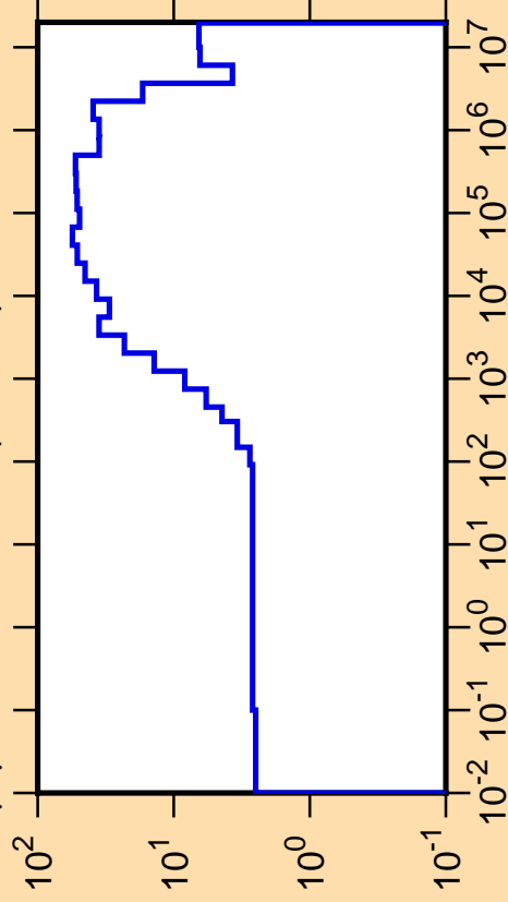
\Delta\mu/\mu vs. E for ^{211}\text{Bi}(\text{mt251})
