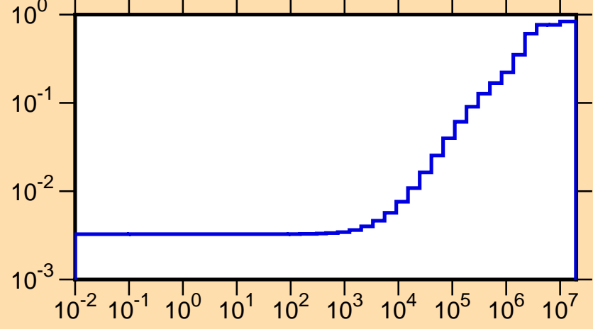
\mu vs. E for ^{211}\text{Bi}(\text{mt251})
