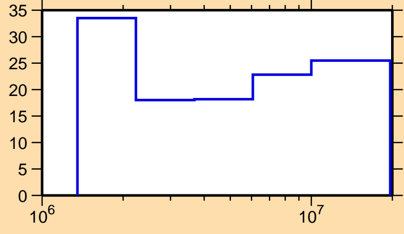
\Delta\sigma/\sigma vs. E for ^{211}\text{Bi}(n,ncont.)
