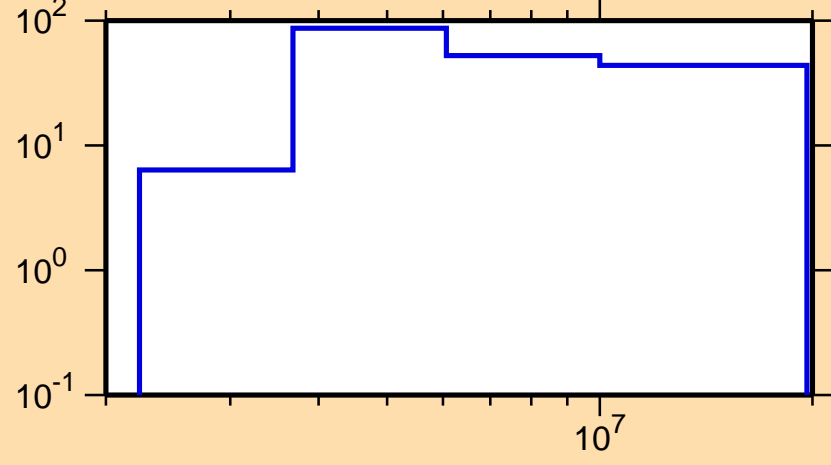
\Delta\sigma/\sigma vs. E for ^{211}\text{Bi}(n,p)
