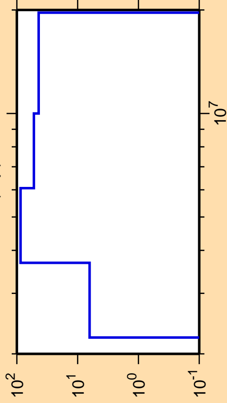
\Delta\sigma/\sigma vs. E for ^{211}\text{Bi}(n,p)
