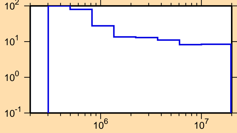
\Delta\sigma/\sigma vs. E for ^{211}\text{Bi}(n,\text{nonel.})
