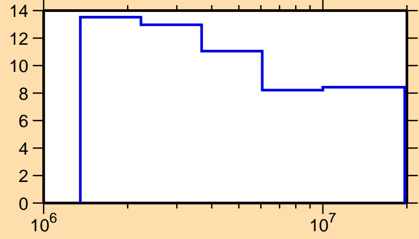
\Delta\sigma/\sigma vs. E for ^{211}\text{Bi}(n,n\text{nonel.})
