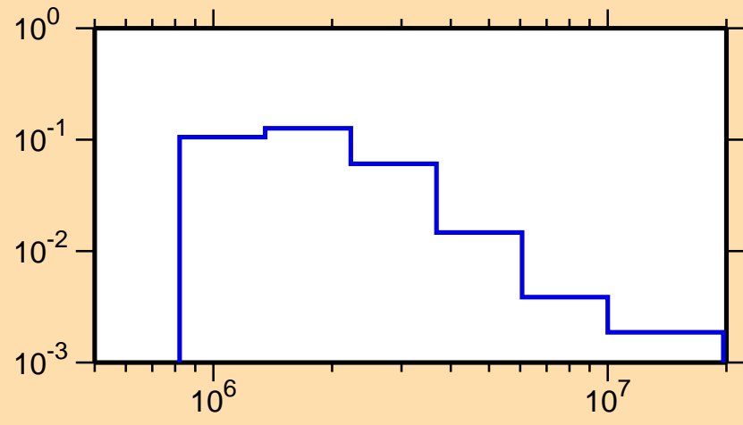
\sigma vs. E for ^{211}\text{Bi}(n,n_4)
