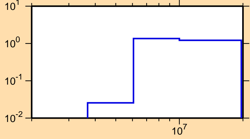
\sigma vs. E for ^{211}\text{Bi}(n,2n)
