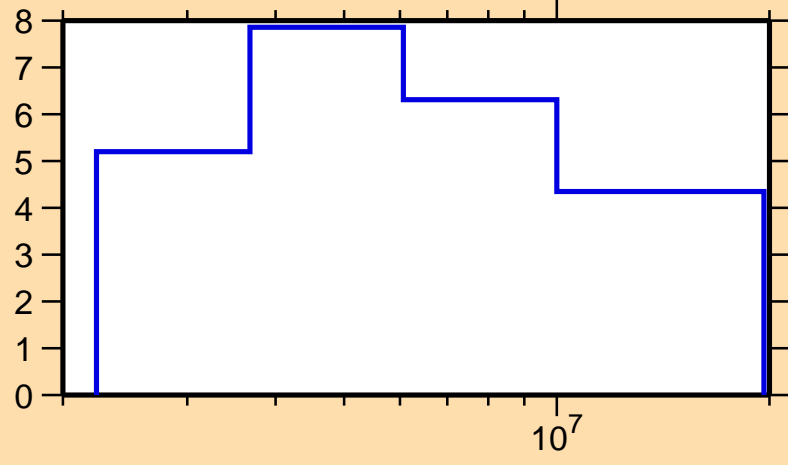
\Delta\sigma/\sigma vs. E for ^{211}\text{Bi}(n,\text{tot.})
