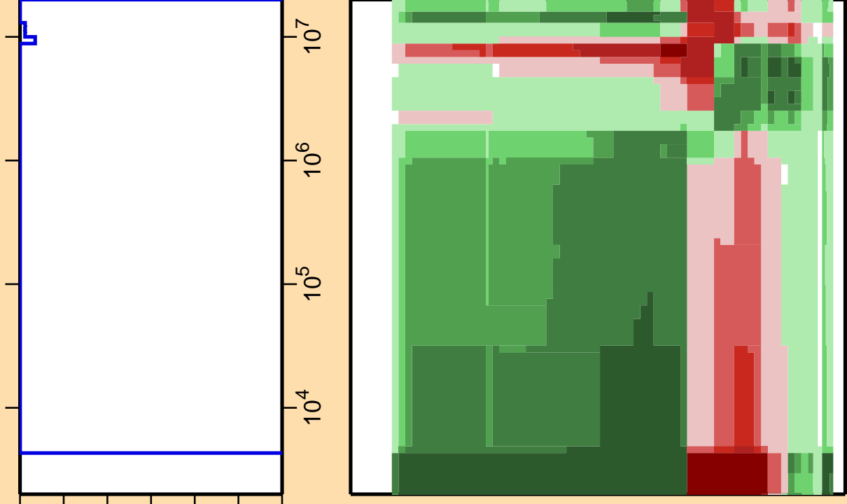
\Delta\sigma/\sigma vs. E for ^{212}\text{Bi}(n,\gamma)
