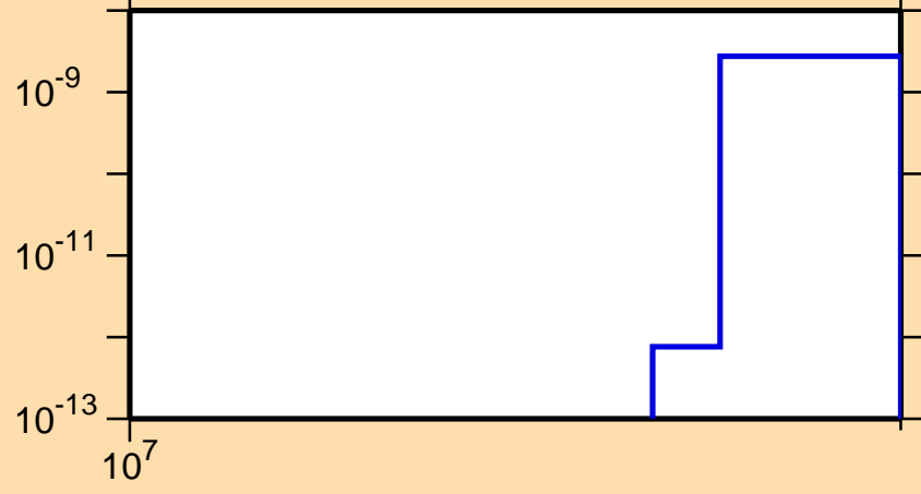
\sigma vs. E for ^{212}\text{Bi} (mt 42)
