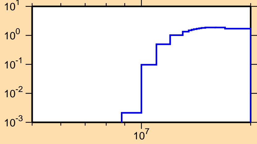
\sigma vs. E for ^{212}\text{Bi}(n,3n)
