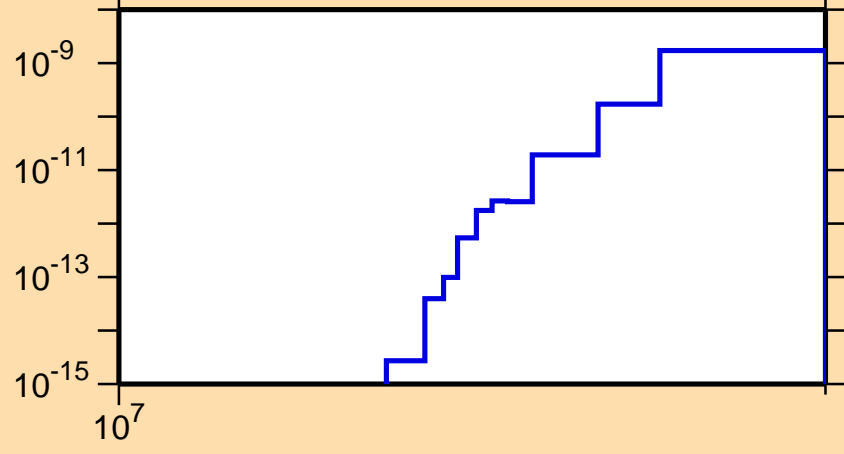
\sigma vs. E for ^{212}\text{Bi}(\text{mt117})
